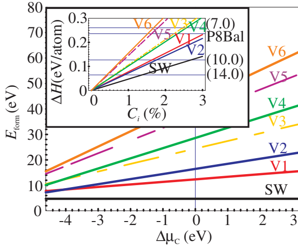
FIG. 2 (color online). Formation energies, E_{\text{form}} , for defects in a graphene sheet as function of \Delta\mu_C = \mu_C - 1/2 E_{C_2} . The right limit is the free C atom at T = 0 K and the left limit is \mu_C of graphene at T = 0 K. The vertical line at \Delta\mu_C = 0 corresponds to the energy of a carbon atom in a C_2 molecule at zero temperature. The labels refer to the SW defect, and the vacancy (V1) and vacancy clusters (from V2 to V6). The inset shows the heat of formation/atom of NPC compared to graphene: \Delta H = H_{\text{NPC}} - H_G as function of the defect concentration. The horizontal lines give \Delta H for three zigzag nanotubes of different diameters (7, 0), (10, 0), and (14, 0) and the P8Bal model of NPC [27].
