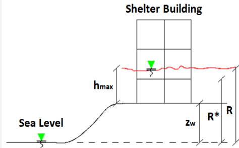
Fig. 5. Inundation of the tsunami plan.
