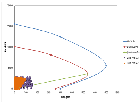
Fig. 6. P-M Interaction diagram of column K1 (Ø 70 cm) at 1 st floor (Interior)
