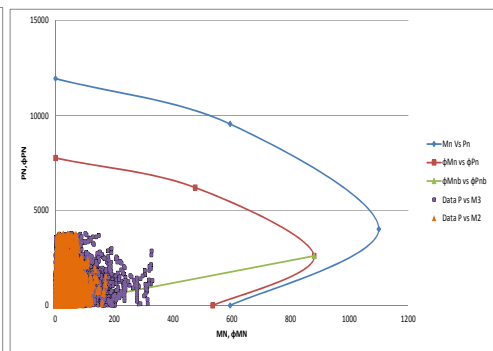
Fig. 7. P-M Interaction diagram of column K2 (Ø 60 cm) at 1 st floor (Exterior)
