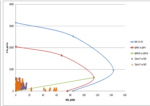
Fig. 9. P-M Interaction diagram of column K4 (Ø 30 cm) at 1 st floor (Exterior)
