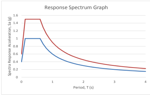
Fig. 4. SD and SF response spectrums.
