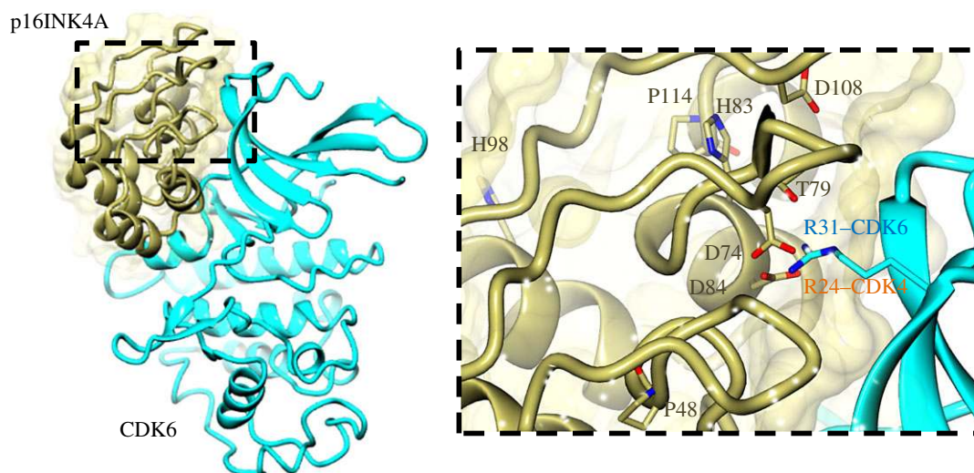
Figure 11. Point mutations in CDK4/6–p16INK4A. CDK4/6 and p16INK4A (represented here by CDK6, PDB 1B17, CDK6, cyan; p16INK4A, gold) contain a number of residues that are frequently mutated in cancer. Several commonly described mutations occur on the CDK–p16INK4A interface, disrupting the complex and leading to kinase dysregulation. Other p16INK4A residues such as H98 and P48 are located further from the CDK-binding interface. CDK6 mutations are selected from those described in cancer genome repositories (see the text for further details).
