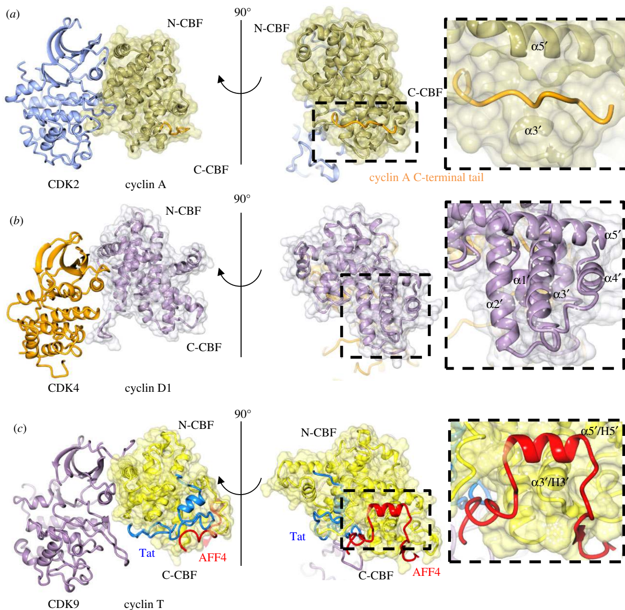
Figure 10. Comparison of cyclin T, cyclin D and cyclin A structures in the vicinity of the AFF4-binding site. (a) CDK2–cyclin A showing the C-CBF with the C-terminal cyclin A tail (orange) accommodated (PDB 1FIN, CDK2–cyclin A coloured as previous). The same site is presented for (b) cyclin D1 (PDB 2W96, coloured as previous) and (c) cyclin T (PDB 40GR, coloured as previous), which is known to accommodate the binding of both AFF4 and Tat.
