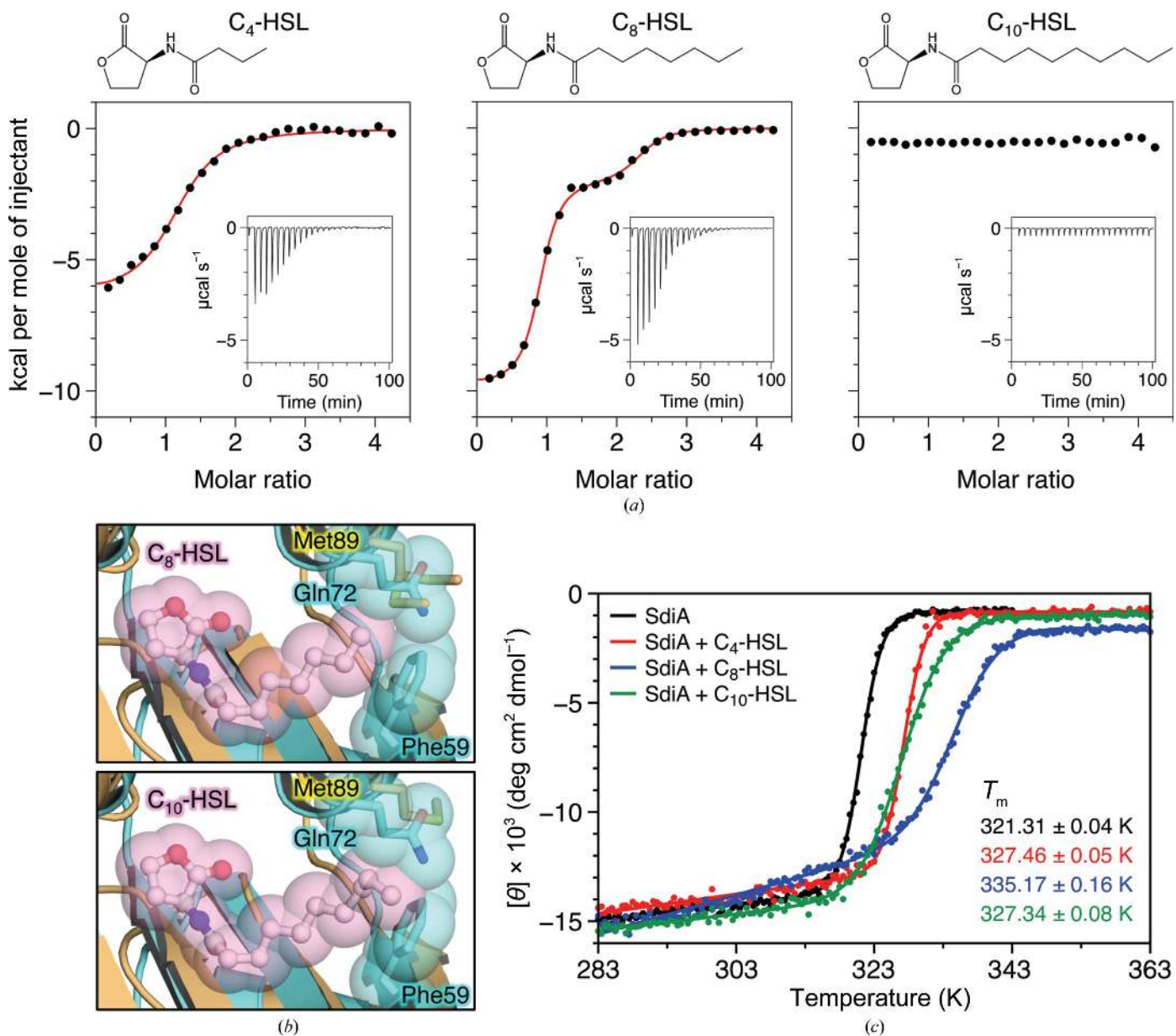
Figure 5 Ligand specificity of SdiA. (a) ITC analyses of different AHLs (drawn at the top) titrated against purified SdiA. The integrated heat exchanges measured at each injection are shown, and the raw data are presented in the inset. The red lines represent nonlinear least-squares data fitting. (b) Structural comparison of the ligand-binding sites of SdiA (cyan) and CviR (orange) in complex with C 8 -HSL (PDB entry 3qp2; left) or C 10 -HSL (PDB entry 3qp4; right). AHLs are illustrated as white ball-and-stick models covered by transparent pink spheres. The side chains of the occlusive residues Phe59 and Gln72 of SdiA and Met89 of CviR are shown as stick models. (c) Thermal stability of SdiA in the presence of different AHLs. The ellipticity changes at 220 nm were monitored from 283 to 343 K and from 283 to 363 K in the absence and presence of AHLs, respectively. The dots represent the raw data and the solid lines depict the fitted curve to calculate the melting temperatures ( T_m ) that are shown in the lower right corner. Data are represented as mean \pm standard error.
