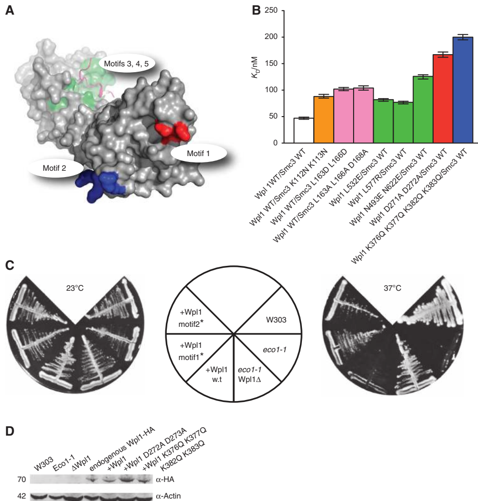
Figure 6 Mutagenesis studies of the Wpl1–Smc3 interaction. (A) Diagram of the Wpl1 domain surface showing the location of the conserved motifs 1–5. (B) Binding constants of ScWpl1 259–647 –ScSmc3AH mutants. The wild-type proteins are shown in white. Other mutants are coloured as follows: Smc3 WIS1—orange, Smc3 WIS2—pink, Wpl1 motifs 3,4,5—green, Wpl1 motif 1—red, Wpl1 motif 2—blue. Error bars are calculated from global fits of data obtained at eight different concentrations. (C) In vivo yeast viability assay of mutants in motifs 1 and 2. All mutants grow at the permissive temperature (left). At the restrictive temperature, mutants in motif 1 (D271A D272A) and motif 2 (K376Q K377Q K382Q K383Q) suppress lethality associated with loss of Eco1 function, indicating Wpl1 inactivation. (D) Cellular expression of the mutant proteins was verified by western blot. Expression levels of the mutant proteins were approximately similar to expression of wild-type Wpl1, both from the HA-tagged endogenous locus (lane 4) and introduced on an integrating plasmid (lane 5).
