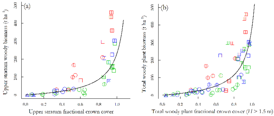
Figure 8. Relationship between (a) biomass and fractional crown cover for the upper-canopy stratum only, and (b) biomass and fractional crown cover for all trees and shrubs taller than 1.5 m. Fitted curves represent a simple reciprocal relationship (viz. 1/y = a + b/x ) and have been fitted using a rank based linear model regression. Symbols as in Fig. 1.
