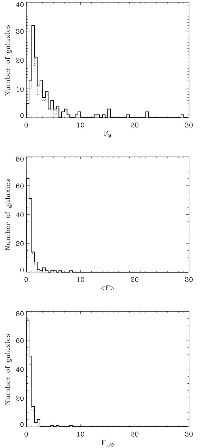
Fig. 5. The distribution of the 148 sample bulges as a function of their maximum ( top panel ), mean ( middle panel ), and median ( bottom panel ) intrinsic flattening, plotted with a solid line. In each panel, the dotted line refers to the distribution of the 115 sample bulges with \phi_C > \phi_M .
