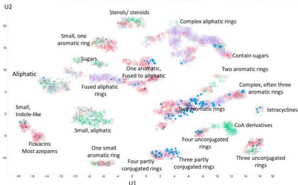
Figure 6. UMAP projection into two dimensions of the four classes of molecules, annotated by the type of molecular structure in the various clusters.
