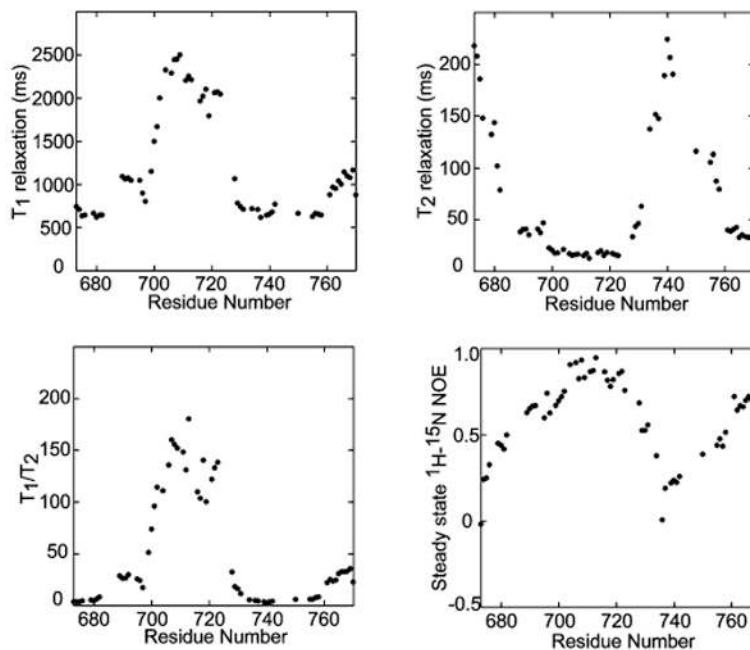
Figure 5. 900 MHz backbone amide ^{15}\text{N} T_1 and T_2 relaxation times and steady-state ^1\text{H} - ^{15}\text{N} NOEs for \text{U-}^{15}\text{N}, ^2\text{H}(70\%)\text{-C99} in LMPG micelles at pH 6.5 and 45 °C.
