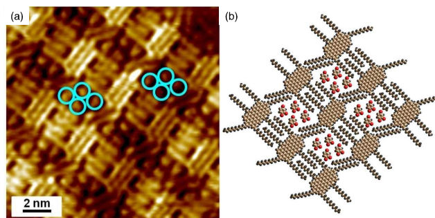
Figure 2. (a) STM image of C78 physisorbed at the Au(111)/TCB interface, blue circles indicate entrapped guest molecules; imaging conditions: I_t = 0.1 nA, V_{bias} = 464 mV. (b) A tentative molecular model for the self-assembly of C78 on Au(111).
