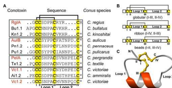
Figure 1. Selected \alpha -conotoxins and their conserved structural framework. (A) Sequences of \alpha -conotoxins that inhibit high voltage-activated (HVA) calcium channel currents ( I_{Ca} ) via the GABA B receptor (in red) and homologous sequences that have been investigated in this study (in black). The boxes indicate groupings of homologous sequences; cysteines are highlighted in yellow and numbered with Roman numerals, and the native CysI - CysIII, CysII - CysIV connectivity is indicated by solid black lines (top). An asterisk indicates an amidated C-terminus. The two loops of the \alpha -conotoxins are indicated at the bottom. (B) A schematic illustration of the three possible disulfide isomers for an \alpha -conotoxin: the globular isomer (CysI - CysIII, CysII - CysIV, top), the ribbon isomer (CysI - CysII, CysIII - CysIV, middle), and the beads isomer (CysI - CysIV, CysII - CysIII, bottom). (C) A 3D ribbon diagram of an \alpha -conotoxin structure showing the N-terminus, C-terminus, and the four loops (I, II, III, IV) connected by disulfide bonds.
