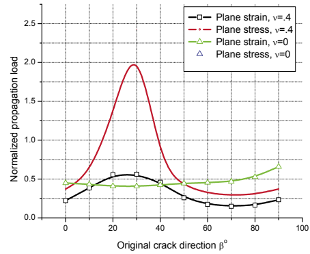
Fig.20 Relation between crack orientation and fracture load.
