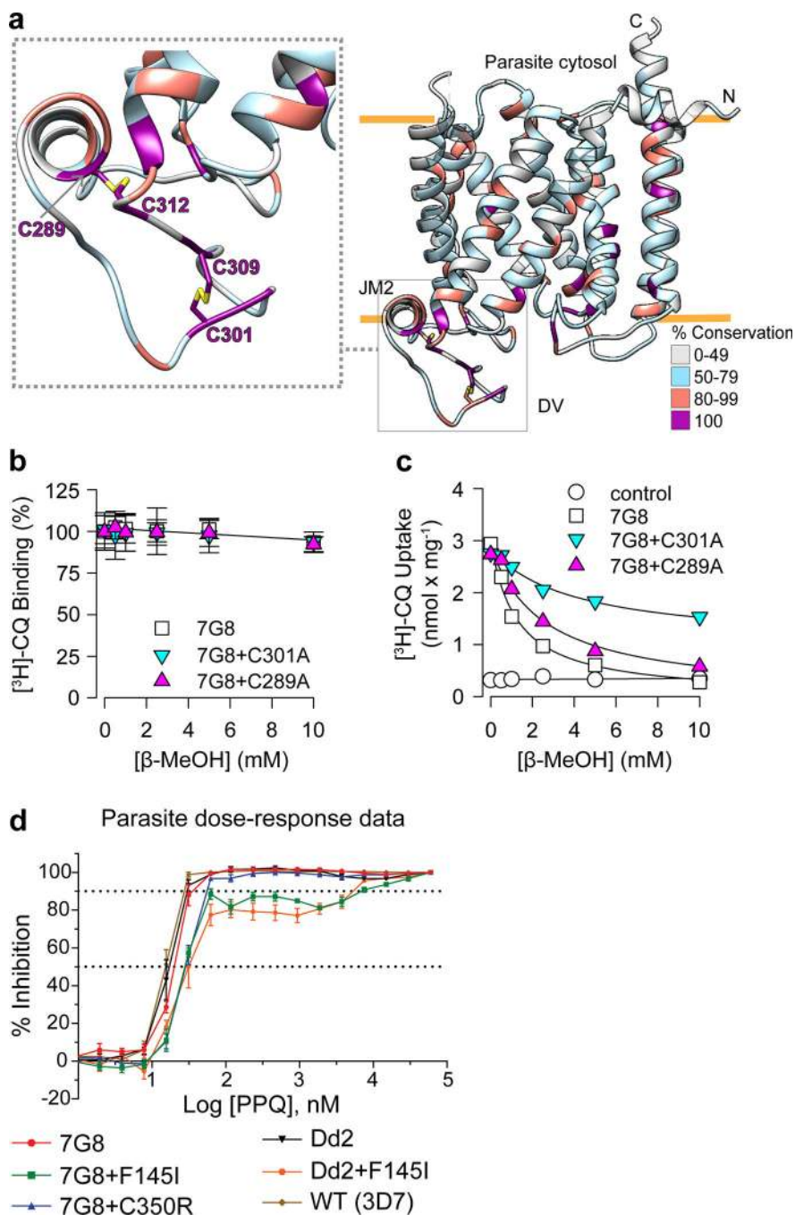
Extended Data Figure 9 | Role of conserved Cys residues in CQ binding and transport, and Parasite PPQ dose-response data.
