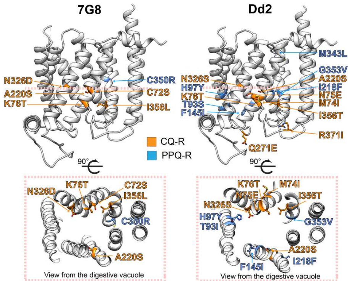
Figure 2 | Mapping of drug-resistance mutations onto the PfCRT structure.
