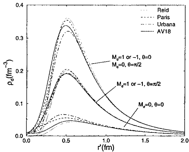
FIG. 36. The top, middle and bottom four curves respectively show the deuteron density \rho_d^{M_d} for the indicated values of M_d and \theta , obtained from various interaction models (Forest et al. , 1996). Note that in the deuteron the two-nucleon density \rho_{T=0, S=1}^{M_d}(\mathbf{r}) = (1/48)\rho_d^{M_d}(\mathbf{r}' = \mathbf{r}/2) .
