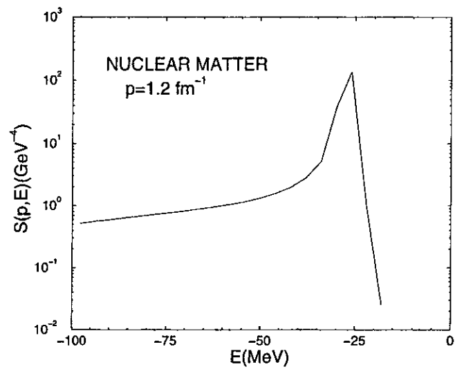
FIG. 50. The hole spectral function for p=1.2 \text{ fm}^{-1} in nuclear matter at equilibrium p_F=1.33 \text{ fm}^{-1} , as obtained Benhar, Fabrocini, and Fantoni (1991)
