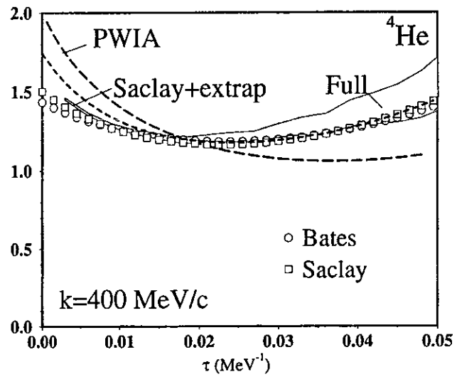
FIG. 71. Scaled Euclidean longitudinal response as in Fig. 69, but for {}^4\text{He} . Data are from Zghiche et al. (1993). Also shown is an estimate of the contribution of the response beyond the experimentally accessible energy.
