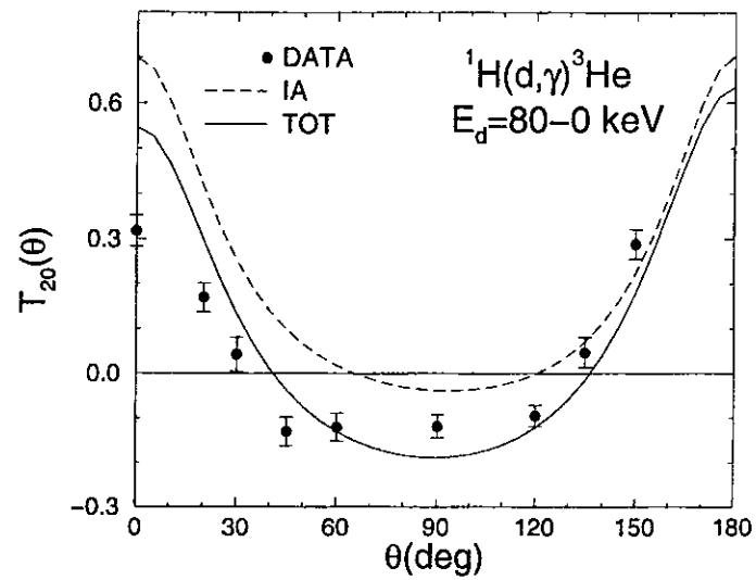
FIG. 57. The energy-integrated tensor analyzing powers of the {}^1\text{H}(d, \gamma){}^3\text{He} reaction, obtained with the AV18/IX Hamiltonian model in impulse approximation (IA) and with inclusion of two-body currents and \Delta -isobar admixtures in the nuclear wave functions (TOT), are compared with experimental results from Schmid et al. (1996).
