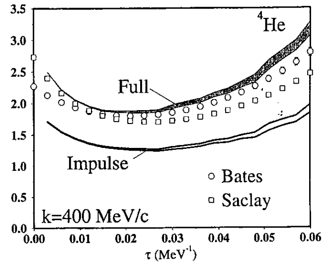
FIG. 72. Transverse Euclidean response as in Fig. 69, but for {}^4\text{He} . Data are from Zghiche et al. (1993).
