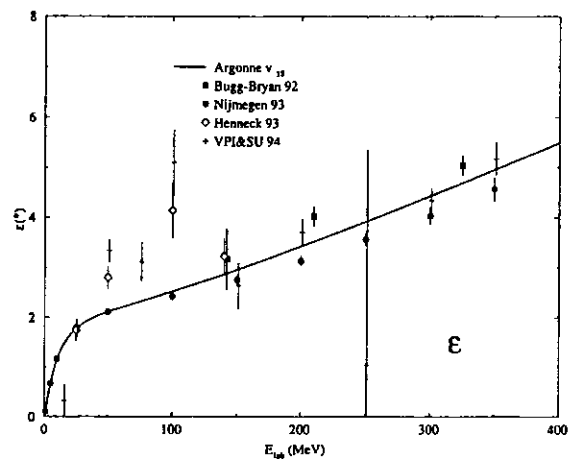
FIG. 4. {}^3S_1 - {}^3D_1 mixing parameter \epsilon_1 from the Argonne v_{18} interaction and various phase shift analyses.
