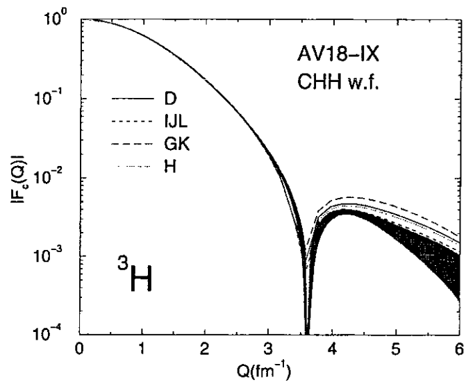
FIG. 30. The {}^3\text{H} charge form factors, calculated with the IJL (Iachello, Jackson, and Lande, 1973), GK (Gari and Krümpelmann, 1986), H (Höhler et al. , 1976), and D (Galster et al. , 1971) parameterizations of the nucleon electromagnetic form factors, are compared with data (shaded area) from Amroun et al. (1994). All theoretical results correspond to the Argonne v_{18} two-nucleon and Urbana IX three-nucleon interactions, use a Correlated-Hyperspherical-Harmonics {}^3\text{H} wave function, and include two-body current contributions and relativistic corrections (Schiavilla and Viviani, 1996).
