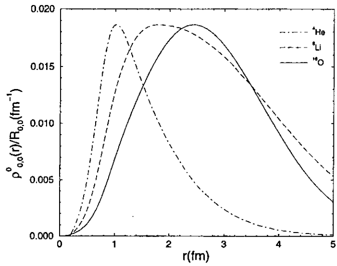
FIG. 42. \rho_{s,0}^0(r)/R_{s,0}^0 for various nuclei (Forest et al., 1996).
