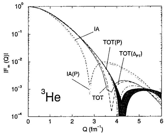
FIG. 26. Same as in Fig. 25, but for {}^3\text{He} .
