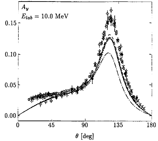
FIG. 61. The nucleon analyzing power A_y for elastic Nd scattering at 10 MeV. 10 MeV: pd data (o) (Sagara et al. , 1994), (x) (Sperisen et al. , 1984), (o) (Rauprich et al. , 1988), and (•) (Clegg and Haeberli, 1967); nd data (o) (Howell et al. , 1987); theory: Nijm I (—), Nijm II (— —), Nijm 93 (— · —), AV18 (· · · · ·), AV14 (— · —), and Nijm 78 (— · ·).
