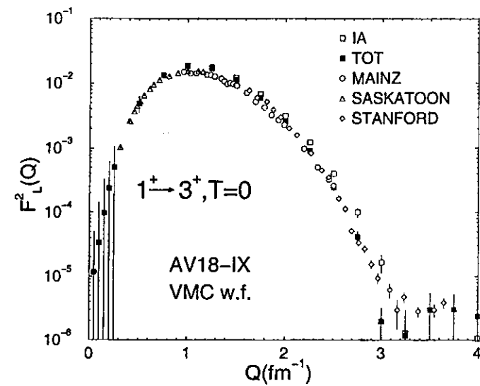
FIG. 33. The longitudinal form factors for the transition from the 1^+, T=0 to the 3^+, T=0 (2.18 MeV) levels of {}^6\text{Li} , obtained in impulse approximation (IA) and with inclusion of two-body charge operator contributions and relativistic corrections (TOT), are compared with data from Bergstrom (1979). The theoretical results correspond to the Argonne v_{18} and Urbana IX three-nucleon interactions, use variational Monte Carlo 1^+, T=0 and 3^+, T=0 {}^6\text{Li} wave functions, and employ the dipole parameterization (including the Galster factor for G_{E,\pi} ) of the nucleon electromagnetic form factors (Wiringa and Schiavilla, 1996).
