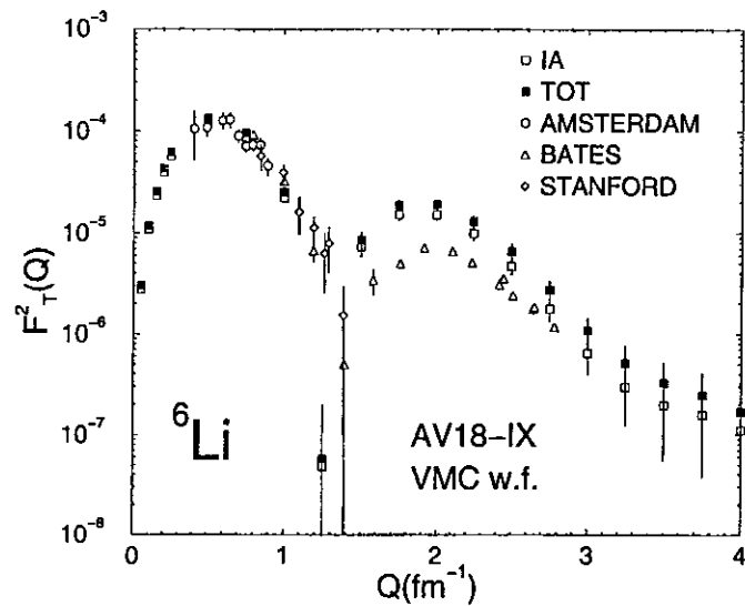
FIG. 32. The transverse form factors of {}^6\text{Li} , obtained in impulse approximation (IA) and with inclusion of two-body current contributions (TOT), are compared with data from Rand, Frosch, and Yearian (1966), /citeasnounLap78, and Bergstrom, Kowalski, and Neuhausen (1982). The theoretical results correspond to the Argonne v_{18} and Urbana IX three-nucleon interactions, use a variational Monte Carlo {}^6\text{Li} wave function, and employ the dipole parameterization (including the Galster factor for G_{E,\pi} ) of the nucleon electromagnetic form factors (Wiringa and Schiavilla, 1996).
