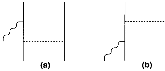
FIG. 16. Feynman diagram representation of the Born amplitudes for photoproduction of virtual mesons. Solid, dashed and wavy lines denote nucleons, mesons, and photons, respectively.
