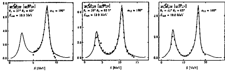
FIG. 64. Breakup cross sections near np FSI peak kinematics. Data at 10 MeV: pd data (o) (Grossman, 1993); 13 MeV: nd data (o) (Strate et al. , 1988; Strate et al. , 1989), pd data (o) (Rauprich et al. , 1991); 19 MeV: pd data (o) (Patberg, 1995). Calculations are for AV18 (—), Nijm 93 (- -), Nijm I (- - -) and Nijm II (· · · · ·) NN interaction models.
