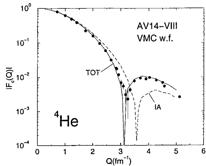
FIG. 29. The charge form factors of {}^4\text{He} , obtained in impulse approximation (IA) and with inclusion of two-body charge contributions and relativistic corrections (TOT), are compared with data from Frosch et al. (1968) and Arnold et al. (1978). Theoretical results correspond to the Argonne v_{14} two-nucleon and Urbana VIII three-nucleon interactions, use a variational Monte Carlo {}^4\text{He} wave function, and employ the dipole parameterization (including the Galster factor for G_{E,\pi} ) for the nucleon electromagnetic form factors (Musolf, Schiavilla, and Donnelly, 1994).
