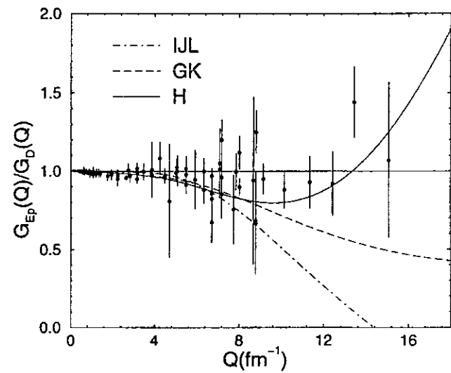
FIG. 9. The proton electric form factor data are compared with the Iachello, Jackson, and Lande (1973) (IJL), Gari and Krümpelmann (1986) (GK), Höhler et al. (1976) (H), and dipole (D) parameterizations. The ratio G_{Ep}/G_D is plotted.
