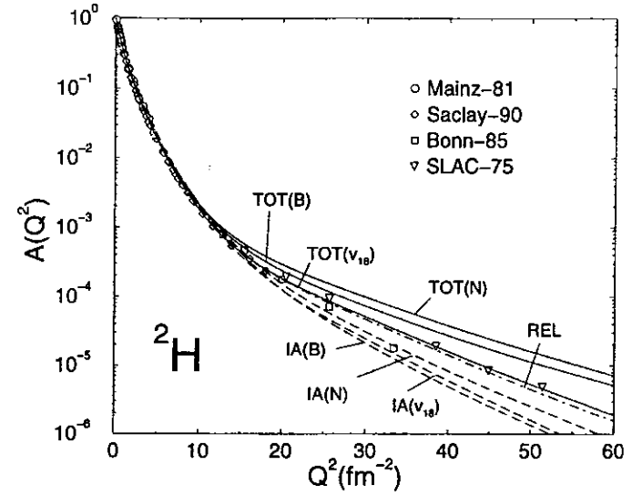
FIG. 21. The deuteron A(Q^2) structure function, obtained in impulse approximation (IA) and with inclusion of two-body charge and current contributions and relativistic corrections (TOT), is compared with data from Simon, Schmitt, and Walther (1981), Cramer et al. (1985), Platchkov et al. (1990), Arnold et al. (1975). Theoretical results corresponding to the Argonne v_{18} ( v_{18} ) (Wiringa, Stoks, and Schiavilla, 1995), Bonn-B (B) (Plessas, Christian, and Wagenbrunn, 1995), and Nijmegen (N) (Plessas, Christian, and Wagenbrunn, 1995) interactions are displayed. Also shown is the relativistically covariant full calculation of Van Orden, Devine, and Gross (1995). The Höhler parameterization is used for the nucleon electromagnetic form factors.
