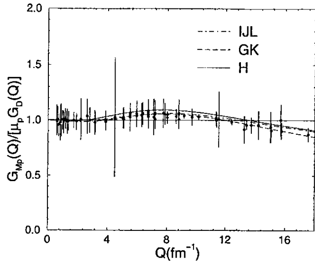
FIG. 10. Same as in Fig. 9, but for the proton magnetic form factor.
