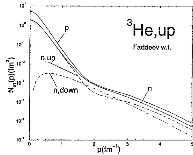
FIG. 47. The proton ( p ), neutron ( n ), neutron spin-up ( n, \text{up} ), neutron spin-down ( n, \text{down} ) momentum distributions in a spin-up {}^3\text{He} nucleus (Carlson and Schivilla, 1997).
