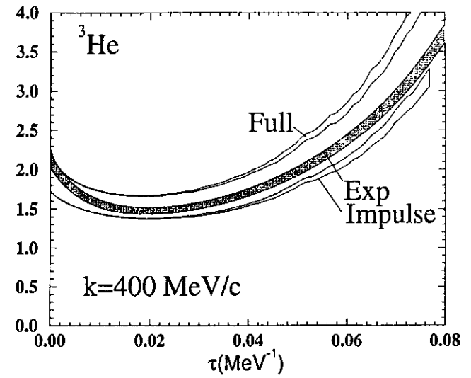
FIG. 70. Scaled Euclidean transverse response of {}^3\text{He} at 400\text{ MeV}/c compared to the Laplace-transform of experimental data from Marchand et al. (1985). The curves marked "impulse" and "full" represent results with single-nucleon and the complete current operators, respectively. In each case the calculations includes a full treatment of final-state interactions.
