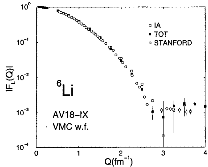
FIG. 31. The longitudinal form factors of {}^6\text{Li} , obtained in impulse approximation (IA) and with inclusion of two-body charge operator contributions and relativistic corrections (TOT), are compared with data from Li et al. (1971). The theoretical results correspond to the Argonne v_{18} and Urbana IX three-nucleon interactions, use a variational Monte Carlo {}^6\text{Li} wave function, and employ the dipole parameterization (including the Galster factor for G_{E,\pi} ) of the nucleon electromagnetic form factors (Wirringa and Schiavilla, 1996).
