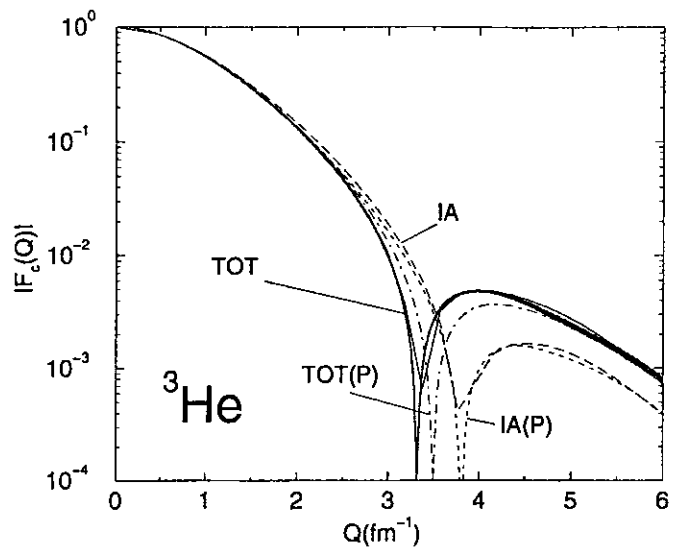
FIG. 28. Same as in Fig. 27, but for {}^3\text{He} .
