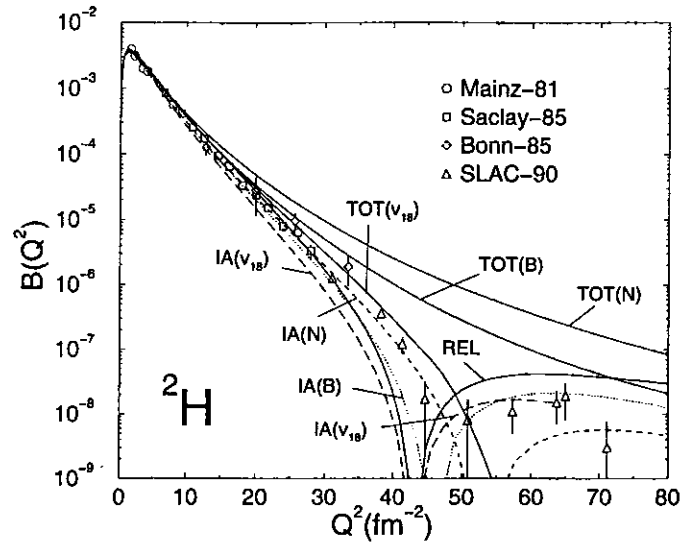
FIG. 20. The deuteron B(Q^2) structure function, obtained in impulse approximation (IA) and with inclusion of two-body current contributions and relativistic corrections (TOT), is compared with data from Simon, Schmitt, and Walther (1981), Cramer et al. (1985), Auffret et al. (1985a), and Arnold et al. (1987). Theoretical results corresponding to the Argonne v_{18} ( v_{18} ) (Wiringa, Stoks, and Schiavilla, 1995), Bonn-B (B) (Plessas, Christian, and Wagenbrunn, 1995), and Nijmegen (N) (Plessas, Christian, and Wagenbrunn, 1995) interactions are displayed. Also shown is the relativistically covariant full calculation of Van Orden, Devine, and Gross (1995). The Höhler parameterization is used for the nucleon electromagnetic form factors.
