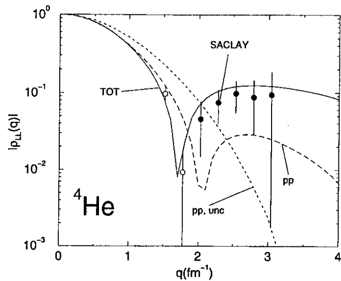
FIG. 46. The experimental longitudinal-longitudinal distribution function (LLDF) of {}^4\text{He} , obtained from the measured charge form factor and tail-corrected Coulomb sum rule data, is compared with theory (Schivilla, Wiringa, and Carlson, 1993). The curve labelled pp only takes into account the proton contributions to the nuclear charge operator, while that labelled TOT also includes the contributions from two-body charge operators and relativistic corrections. Also shown is the LLDF for uncorrelated protons (curve labelled pp, \text{unc} ). Note that the empty and filled circles denote positive and negative values for the experimental LLDF.
