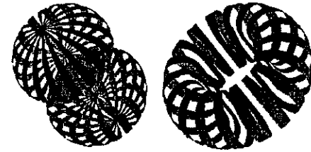
FIG. 1. Nucleon densities of the S=1 deuteron in its two spin projections, S_z=\pm 1 and S_z=0 , respectively.
