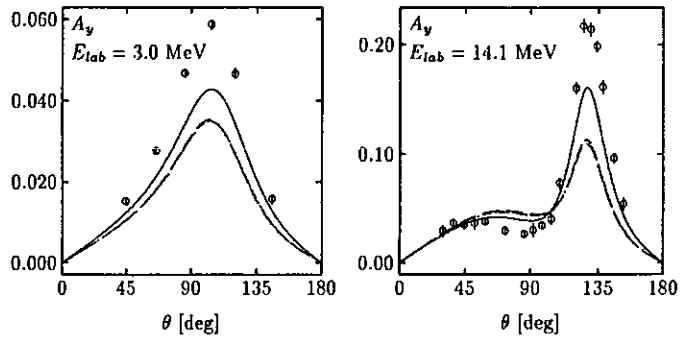
FIG. 62. Comparison of A_y data with results obtained from the Bonn-B NN interaction model plus Tucson-Melbourne three-nucleon interaction, \pi\text{-}\pi (---), \pi\text{-}\pi+\pi\text{-}p (- - -), and \pi\text{-}\pi+\pi\text{-}p+p\text{-}p (.....). The nd data are from (McAninch et al. , 1993), (McAninch, Lamm, and Haerberli, 1994) (3 MeV), and (Howell et al. , 1987) (14.1 MeV).
