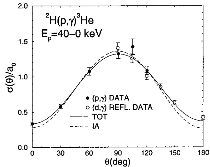
FIG. 55. The energy-integrated relative cross sections, \sigma(\theta)/a_0 ( 4\pi a_0 is the total cross section), obtained with the AV18/IX Hamiltonian model in impulse approximation (IA) and with inclusion of two-body currents and \Delta -isobar admixtures in the nuclear wave functions (TOT), are compared with experimental results from Schmid et al. (1996). Note that this plot only shows data with E_p = 0-40 keV ( E_{CM} = 0-27 keV). This is done to allow the (d,\gamma) data with E_d = 0-80 keV ( E_{CM} = 0-27 keV) and the (p,\gamma) data to be shown in the same graph (with the (d,\gamma) data reflected).
