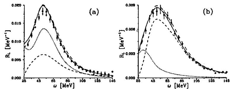
FIG. 68. {}^3\text{He} (a) and {}^3\text{H} (b) longitudinal response at 300 MeV/c, as in Fig. 67.
