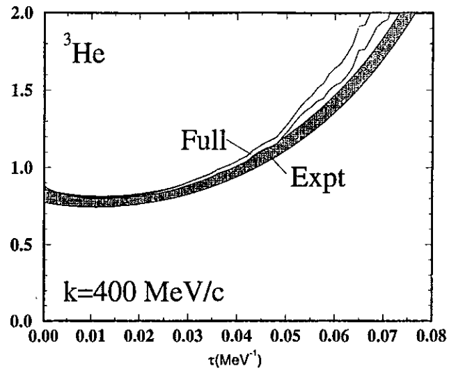
FIG. 69. Scaled Euclidean longitudinal response of {}^3\text{He} at 400\text{ MeV}/c compared to the Laplace-transform of experimental data from Marchand et al. (1985). The shaded bands represent the approximate experimental uncertainty and statistical errors in the Monte Carlo calculation.
