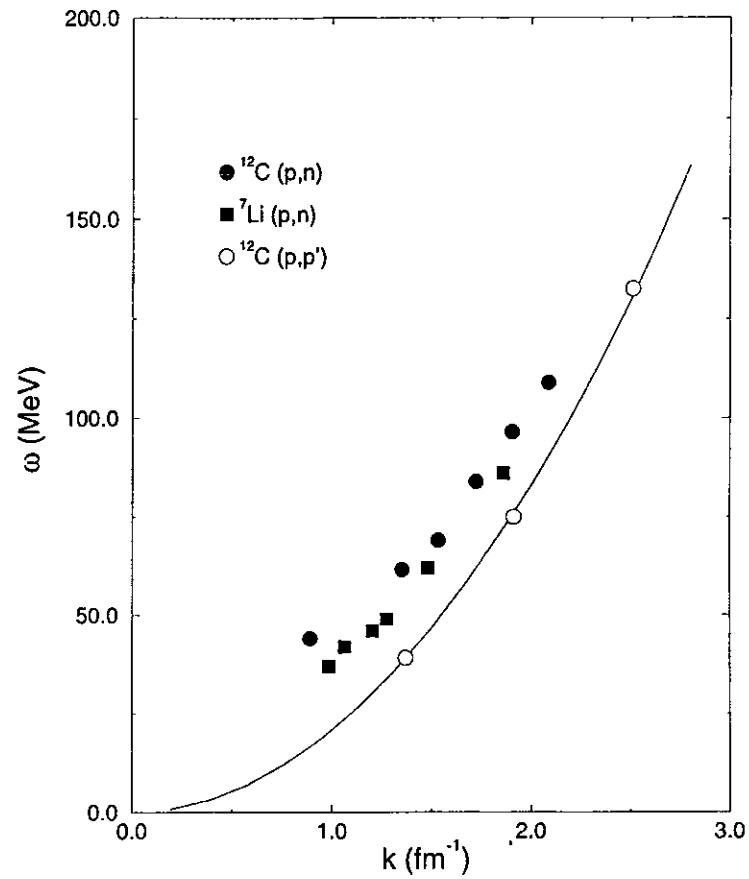
FIG. 74. Peak position measured for quasielastic scattering with different experiments. The solid line is the free-particle peak position.
