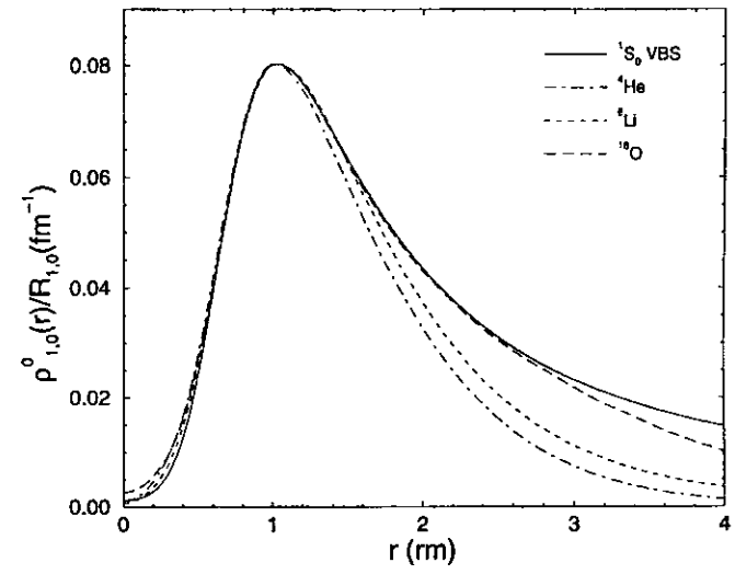
FIG. 43. \rho_{p,0}^0(r)/R_{p,0}^0 for various nuclei (Forest et al., 1996).
