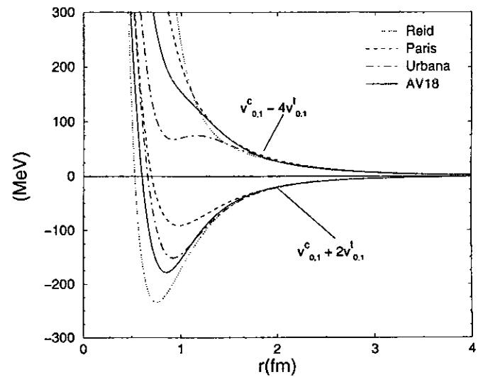
FIG. 35. The upper four lines show expectation values of v_{0,1}^{c, \pm 1} for M_S=0, \theta=0 , and the lower four lines are for M_S=0, \theta=\pi/2 or equivalently M_S=\pm 1, \theta=0 . The expectation values for M_S=\pm 1, \theta=\pi/2 (not shown) are half way in between.
