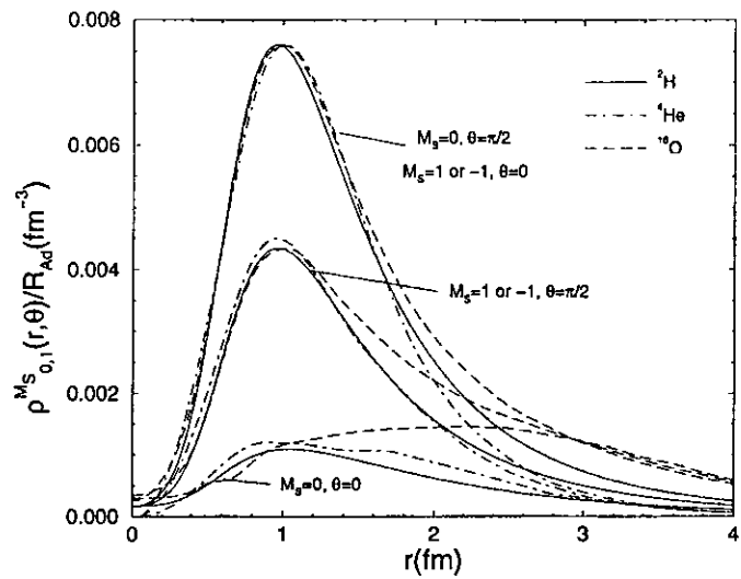
FIG. 40. \rho_{T=0,S=1}^{M_S}(r,\theta)/R_{Ad} for various nuclei (Forest et al. , 1996).
