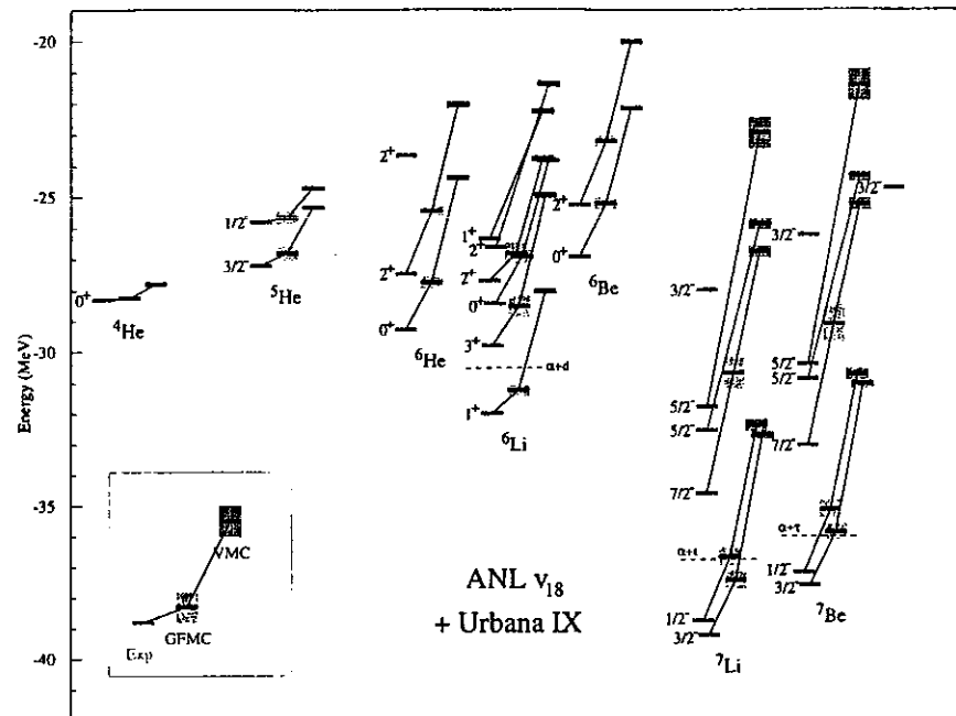
FIG. 7. Energy spectra of A=4-7 nuclei, obtained in VMC and GFMC calculations with the Argonne v_{18} two-nucleon and Urbana model IX three-nucleon interactions. Both the central value and the one-standard deviation error estimate are shown. GFMC results are a variational bound obtained by averaging from \tau=0.04-0.06 \text{ MeV}^{-1} .
