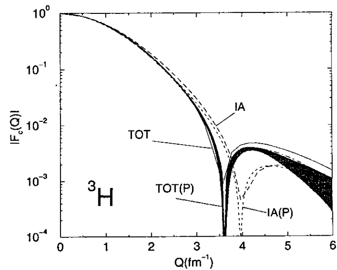
FIG. 27. The charge form factors of {}^3\text{H} , obtained in impulse approximation (IA) and with inclusion of two-body charge contributions and relativistic corrections (TOT), are compared with data (shaded area) from Amroun et al. (1994). Theoretical results correspond to the Argonne v_{18} two-nucleon and Urbana IX three-nucleon (Schiavilla and Viviani, 1996) and Paris two-nucleon (P) (Struewe et al. , 1987) interactions, use, respectively, Correlated-Hyperspherical-Harmonics and Faddeev wave functions, and employ the dipole parameterization (including the Galster factor for G_{E,p} ) for the nucleon electromagnetic form factors. Note that the Paris-based calculation also includes \Delta -isobar admixtures in the {}^3\text{H} wave function.
