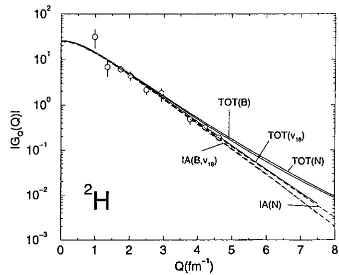
FIG. 19. Same as in Fig. 18, but for the quadrupole form factor of the deuteron.
