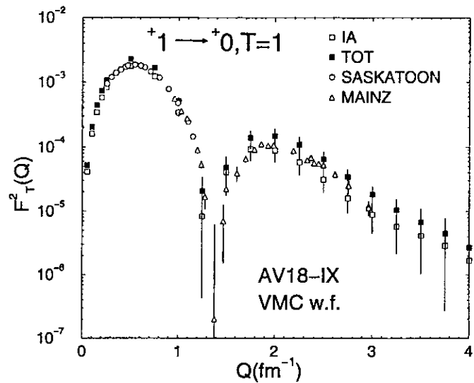
FIG. 34. The transverse form factors for the transition from the 1^+, T=0 to the 0^+, T=1 (3.56 MeV) levels of {}^6\text{Li} , obtained in impulse approximation (IA) and with inclusion of two-body current contributions (TOT), are compared with data from Bergstrom, Deutschmann, and Neuhausen (1979). The theoretical results correspond to the Argonne v_{18} and Urbana IX three-nucleon interactions, use variational Monte Carlo 1^+, T=0 and 0^+, T=1 {}^6\text{Li} wave functions, and employ the dipole parameterization (including the Galster factor for G_{E,\pi} ) of the nucleon electromagnetic form factors Wiringa and Schiavilla (1996).
