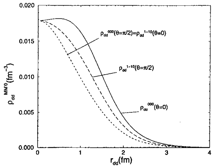
FIG. 44. Density distributions of dd clusters in {}^4\text{He} in parallel ( \theta=0 ) and transverse ( \theta=\pi/2 ) directions (Forest et al. , 1996).
