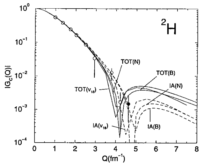
FIG. 18. The charge form factor of the deuteron, obtained in impulse approximation (IA) and with inclusion of two-body charge contributions and relativistic corrections (TOT), is compared with data from Schulze et al. (1984), The et al. (1991), Dmitriev et al. (1985), Gilman et al. (1990) (empty and filled circles denote, respectively, positive and negative experimental values for G_C(Q) ). Theoretical results corresponding to the Argonne v_{18} ( v_{18} ) (Wirringa, Stoks, and Schiavilla, 1995), Bonn-B (B) (Plessas, Christian, and Wagenbrunn, 1995), and Nijmegen (N) (Plessas, Christian, and Wagenbrunn, 1995) interactions are displayed. The Höhler parameterization is used for the nucleon electromagnetic form factors.
