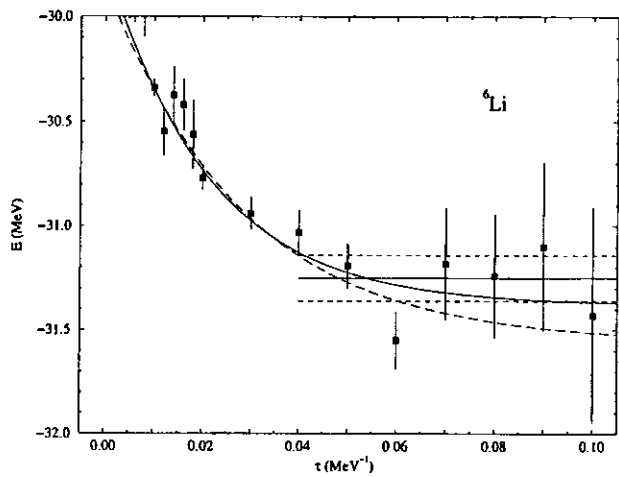
FIG. 8. Convergence with imaginary time \tau of the GFMC calculations of A=6 . Curves are fits based to ground-state plus excitations, and the horizontal lines are the average from \tau = 0.04\text{-}0.06 \text{ MeV}^{-1} plus and minus one standard deviation.
