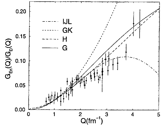
FIG. 11. The neutron electric form factor data are compared with Iachello, Jackson, and Lande (1973) (IJL), Gari and Krümpelmann (1986) (GK), Höhler et al. (1976) (H), and Galster et al. (1971) (G) parameterizations. The ratio G_{E_n}/G_D is plotted.
