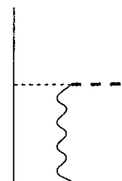
FIG. 14. Feynman diagram representation of the isoscalar \rho\pi\gamma and isovector \omega\pi\gamma transition currents. Solid, dashed, thick-dashed, and wavy lines denote nucleons, pions, vector mesons (either \rho or \omega ), and photons, respectively.
