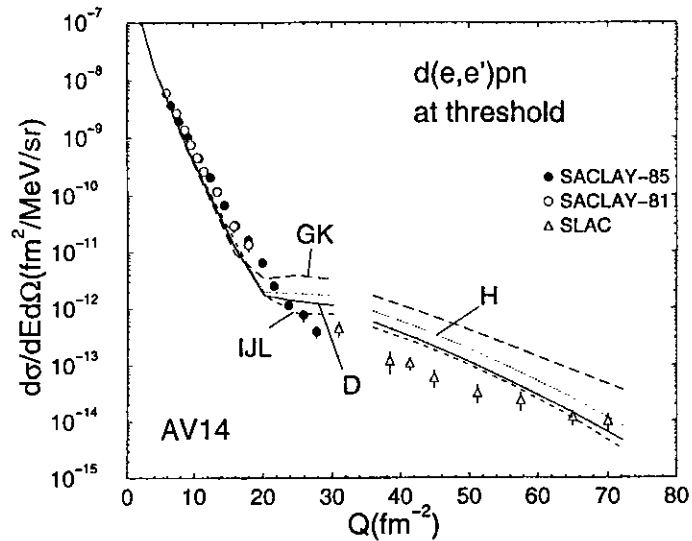
FIG. 24 The cross sections for backward electrodisintegration of the deuteron near threshold, obtained with the IJL (Iachello, Jackson, and Lande, 1973), GK (Gari and Krümpelmann, 1986), H (Höhler et al. , 1976), and D (Galster et al. , 1971) parameterizations of the nucleon electromagnetic form factors, are compared with data from Cox, Wyachank, and Collie (1965), Bernheim et al. (1981), Auffret et al. (1985b), Arnold et al. (1990). All theoretical results correspond to the Argonne v_{14} interaction, and include two-body current contributions and relativistic corrections (Schiavilla and Riska, 1991). The Sachs form factor G_2^V(Q^2) is used in the isovector model-independent two-body current operators.
