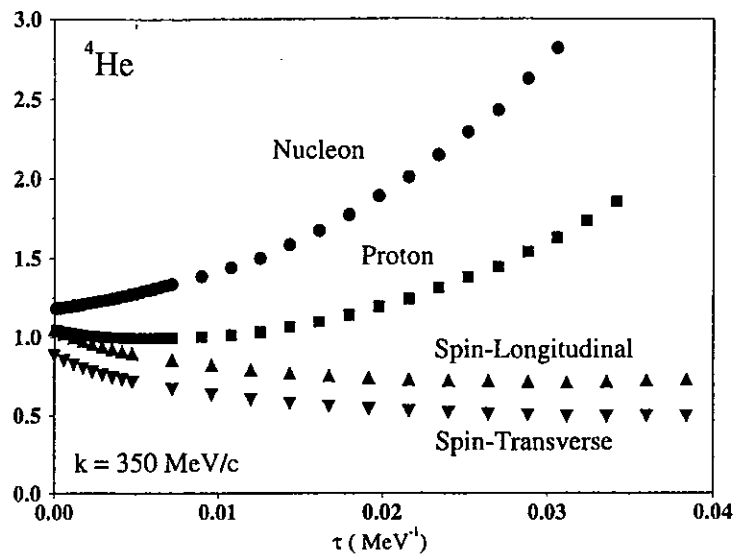
FIG. 73. Scaled Euclidean response for a variety of idealized single-nucleon couplings in the \alpha -particle.
