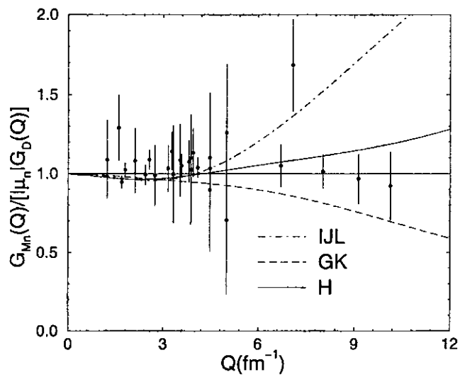
FIG. 12. Same as in Fig. 9, but for the neutron magnetic form factor.
