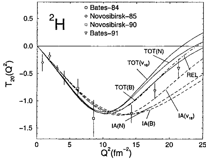
FIG. 22. The deuteron tensor polarization T_{20}(Q^2) , obtained in impulse approximation (IA) and with inclusion of two-body charge and current contributions and relativistic corrections (TOT), is compared with data from Schulze et al. (1984), The et al. (1991), Dmitriev et al. (1985), Gilman et al. (1990). Theoretical results corresponding to the Argonne v_{18} ( v_{18} ) (Wirring, Stoks, and Schiavilla, 1995), Bonn-B (B) (Plessas, Christian, and Wagenbrunn, 1995), and Nijmegen (N) (Plessas, Christian, and Wagenbrunn, 1995) interactions are displayed. Also shown is the relativistically covariant full calculation of Van Orden, Devine, and Gross (1995). The Höhler parameterization is used for the nucleon electromagnetic form factors.
