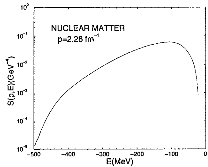
FIG. 51. The hole spectral function for p=2.26 \text{ fm}^{-1} in nuclear matter at equilibrium p_F=1.33 \text{ fm}^{-1} , as obtained Benhar, Fabrocini, and Fantoni (1991).
