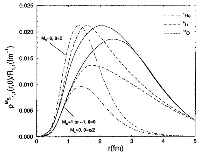
FIG. 41. \rho_{l=1}^{M_S}(r,\theta)/R_{l=1}^A for various nuclei (Forest et al. , 1996). The upper three curves are for M_S=0, \theta=0 while the lower ones are for M_S=0, \theta=\pi/2 and equivalently M_S=\pm 1, \theta=0 .
