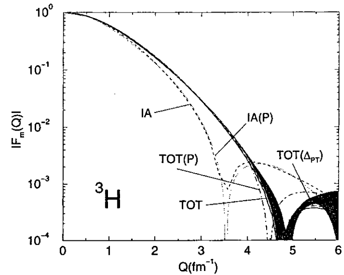
FIG. 25. The magnetic form factors of {}^3\text{H} , obtained in impulse approximation (IA) and with inclusion of two-body current contributions and \Delta admixtures in the bound-state wave function (TOT), are compared with data (shaded area) from Amroun et al. (1994). Theoretical results correspond to the Argonne v_{14} two-nucleon and Urbana IX three-nucleon (Schiavilla and Viviani, 1996) and Paris two-nucleon (P) (Struerve et al. , 1987) interactions, use, respectively, Correlated-Hyperspherical-Harmonics and Faddeev wave functions, and employ the dipole parameterization (including the Galster factor for G_{E,n} ) for the nucleon electromagnetic form factors. Note that the Sachs form factor G_2^V(Q^2) (Dirac form factor F_1^V(Q^2) ) is used in the isovector model-independent two-body current operators for the Argonne-based (Paris-based) calculations. Also shown are the Argonne results (curve labelled TOT( \Delta_{PT} ) obtained by including the two-body currents associated with intermediate excitation of a single \Delta -isobar in perturbation theory.
