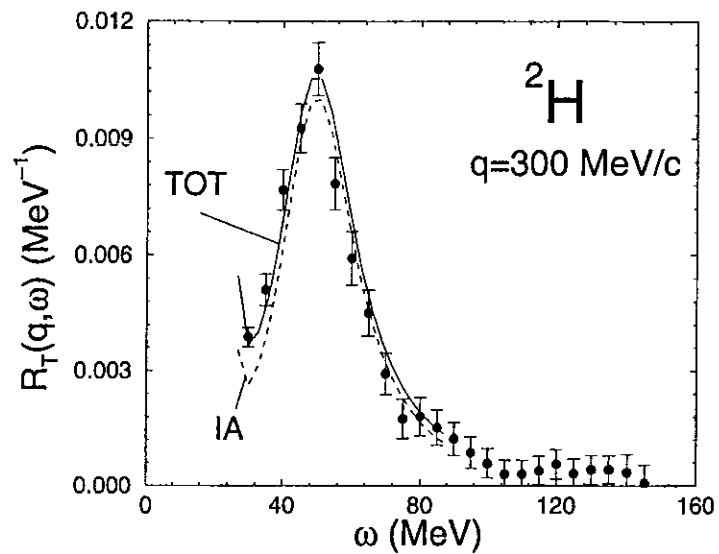
FIG. 66. Deuteron transverse response at 300 MeV/c, as in Fig. 65.
