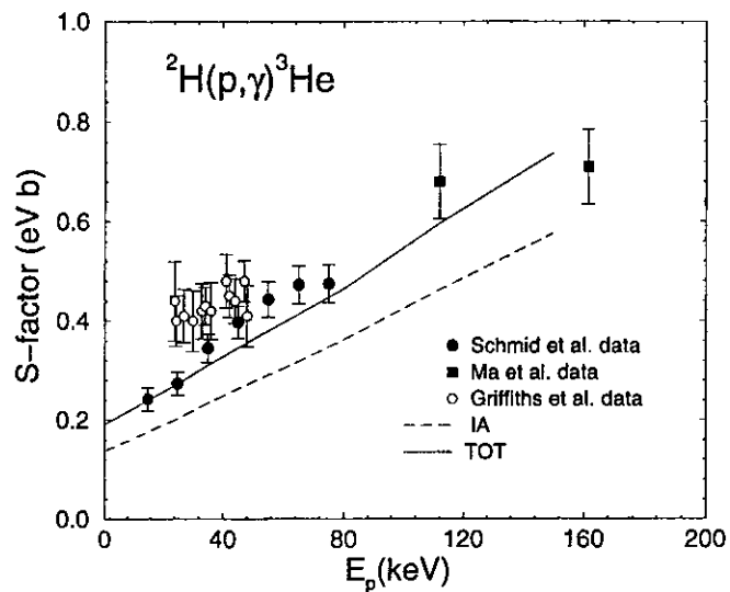
FIG. 54. The S -factor of the {}^2\text{H}(p,\gamma){}^3\text{He} reaction, obtained with the AV18/IX Hamiltonian model in impulse approximation (IA) and with inclusion of two-body currents and \Delta -isobar admixtures in the nuclear wave functions (TOT), is compared with experimental results from Griffiths, Lal, and Scarfe (1963), Schmid et al. (1996) and Ma et al. (1996).
