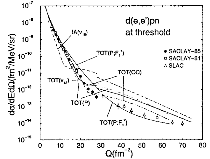
FIG. 23. The cross sections for backward electrodisintegration of the deuteron near threshold, obtained in impulse approximation (IA) and with inclusion of two-body current contributions and relativistic corrections (TOT), are compared with data from Cox, Wynchank, and Collie (1965), Bernheim et al. (1981), Auffret et al. (1985b), Arnold et al. (1980). Theoretical results corresponding to the Argonne v_{18} ( v_{18} ) (Schiavilla, 1996), Paris (P) (Leidemann, Schmitt, and Arenhövel, 1990), and r -space version C of the Bonn (QC) (Leidemann, Schmitt, and Arenhövel, 1990) interactions are displayed. The dipole parameterization (including the Galster factor for G_{E,N} ) is used for the nucleon electromagnetic form factors; in particular, the Sachs form factor G_E^N(Q^2) is used in the isovector model-independent two-body current operators. For the Paris interaction, the results obtained by using the Dirac form factor F_1^V(Q^2) in these two-body currents are also shown (curve labelled TOT(P; F_1^V )).
