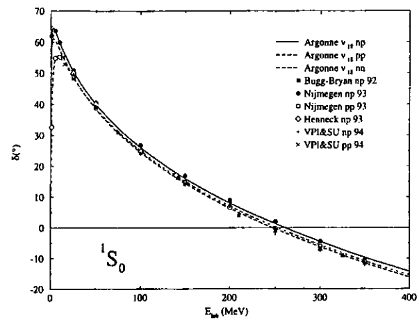
FIG. 3. ^1S_0 phases of the Argonne v_{18} interaction compared to various np and pp phase shift analyses.
