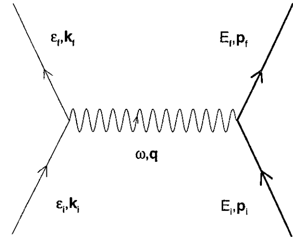
FIG. 17. Electron scattering in the one-photon exchange approximation. Solid, thick-solid and wavy lines denote electrons, hadrons, and photons, respectively.
