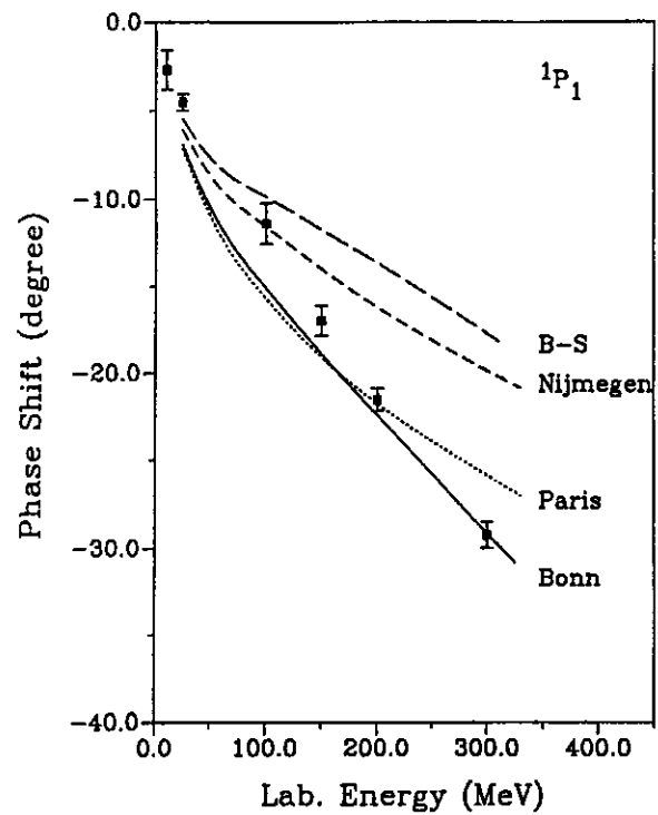
FIG. 2. Singlet ^1P_1 phases in a variety of previous-generation interaction models. Not all interactions have been fit to the same data.
