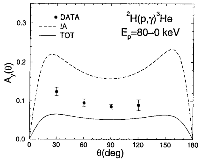
FIG. 56. The energy-integrated vector analyzing powers of the {}^2\text{H}(p, \gamma){}^3\text{He} reaction, obtained with the AV18/IX Hamiltonian model in impulse approximation (IA) and with inclusion of two-body currents and \Delta -isobar admixtures in the nuclear wave functions (TOT), are compared with experimental results from Schmid et al. (1996).
