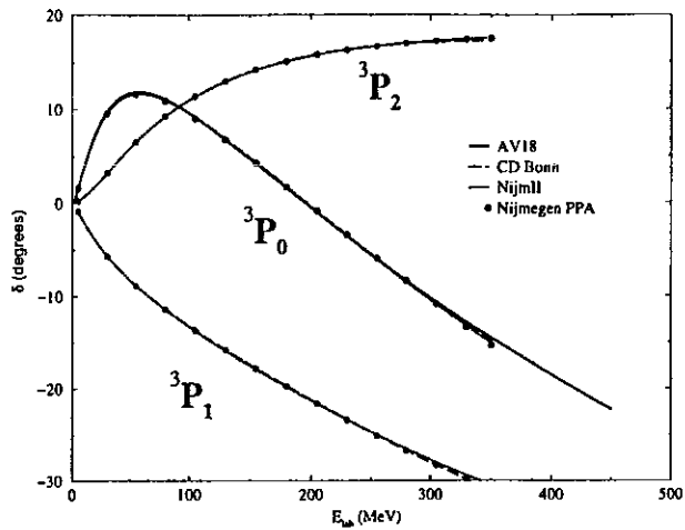
FIG. 6. {}^3P_J phases from different modern NN interaction models.
