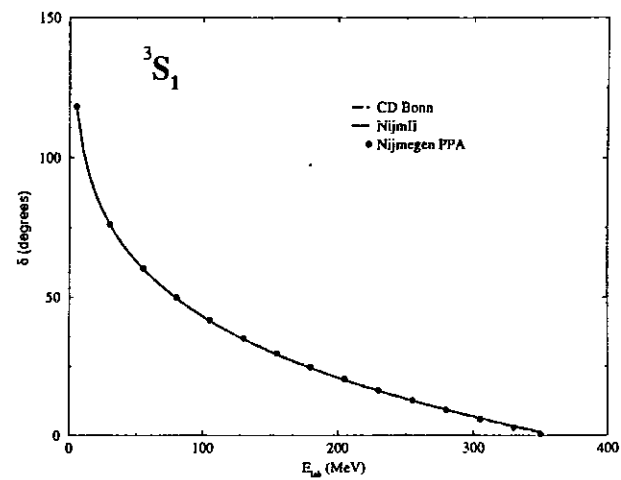
FIG. 5. {}^3S_1 phases from different modern NN interaction models.
