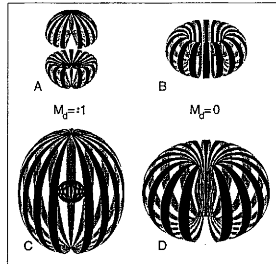
FIG. 39. The surfaces having \rho_d^{M_d=\pm 1}(r')=0.24 \text{ fm}^{-3} (A) and \rho_d^{M_d=0}(r')=0.24 \text{ fm}^{-3} (B). The surfaces are symmetric about z' axis and have r' \leq 0.74 \text{ fm} , i.e., the length of the dumbbell along z' axis as well as the diameter of the outer surface of the torus is 1.48 fm. Sections C and D are for \rho_d^{M_d=\pm 1, 0}(r')=0.08 \text{ fm}^{-3} ; the maximum value of r' is 1.2 fm (Forest et al. , 1996). Note that in the deuteron the two-nucleon density \rho_{T=0, S=1}^{M_d}(r) = (1/48)\rho_d^{M_d=M_d}(r' = r/2) .
