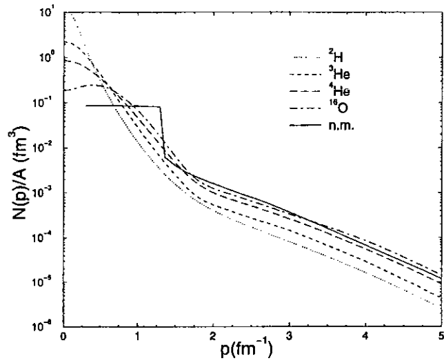
FIG. 48. The N(p) = \sum_{\sigma, \tau} N_{\sigma, \tau}(p) per nucleon in ^2\text{H} , ^3\text{He} , ^4\text{He} , ^{16}\text{O} , and nuclear matter (n.m.) (Pieper, Wiringa and Pandharipande, 1992).
