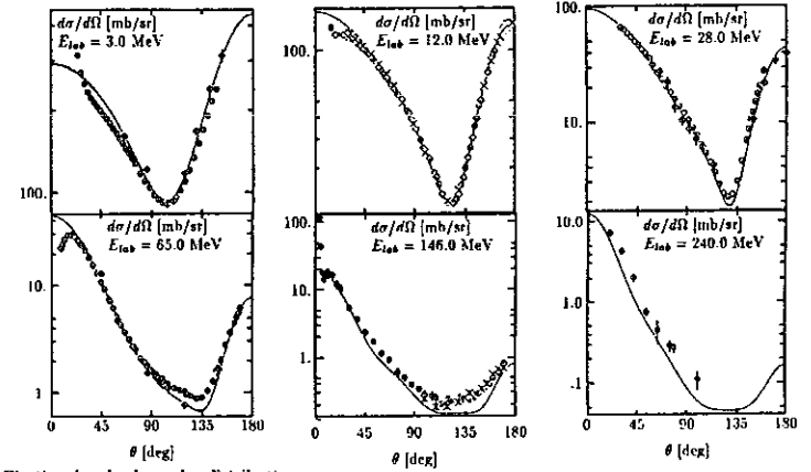
FIG. 59. Elastic pd and nd angular distributions. 3 MeV: pd data (o) (Sagara et al. , 1994); nd data (o) (Schwarz, et al. , 1983); theory: Nijm I (—), Nijm II (- -), Nim 93 (- · - ·), and AV18 (· · · · ·). 12 MeV: pd data (o) (Sagara et al. , 1994), (o) (Gruebler et al. , 1983), (x) (Rauprich et al. , 1988); theory: AV18 (—). 28 MeV: pd data (o) (Hatanaka et al. , 1984); nd data (o) (Gouanere et al. , 1970); theory: Nijm I (—). 65 MeV: pd data (o) (Shimizu, et al. , 1982); nd data (o) (Rühi et al. , 1991); theory: AV18 (—). 146 MeV: pd data (o) (Postma and Wilson, 1961), (o) (Igo, G. et al. , 1972); nd data at 152 MeV (x) (Palmieri, 1972); theory: AV18 (—). 240 MeV: pd data (o) (Schamberger, 1952); theory: AV18 (—).
