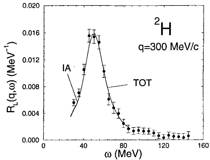
FIG. 65. Deuteron longitudinal response at 300 MeV/c, theory from Carlson and Schiavilla (1992) and experiment from Dytman et al. (1988). Calculations include FSI and show results with one- and two-body charge operators.
