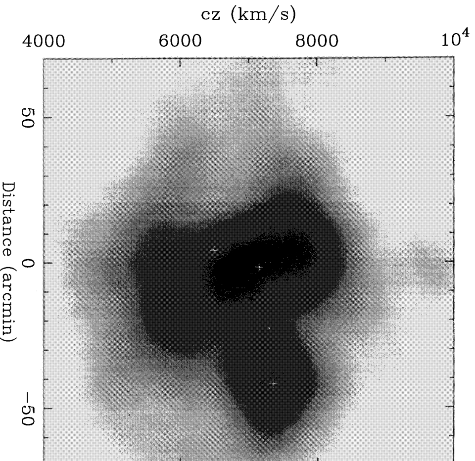
FIG. 10—Galaxy density distribution projected onto the plane of radial velocity versus projected distance from the cluster center along the NE-SW diagonal (NE positive). The density is smoothed with a Gaussian of dispersion 8' in the spatial dimension and 300 \text{ km s}^{-1} in the velocity dimension. The positions of the three dominant galaxies are marked by crosses [left to right: NGC 4889, NGC 4874, NGC 4839]. The gray scale is linear with density and runs from zero to the maximum.
