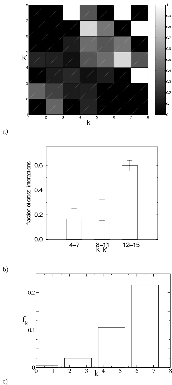
Figure 3 Link attachment occurs preferentially towards proteins of high connectivity. (a) The color-coded plot shows the fraction of duplicate pairs with connectivities ( k, k' ) that have gained a mutual interaction (cross-interaction) since duplication, as a function of k and k' . Points where all duplicate pairs have cross-interactions are shown in white, points where none carry a cross-interactions are shown black. Points (particularly at high connectivities) where no data is available are also shown in black. The number of duplicate pairs with given connectivities ranges from 2 to 39. Points in the k, k' -plane where only a single pair of duplicates exists are excluded. (b) For this histogram the data from a) are binned for low, medium, and high k + k' and the average for each bin is shown against k + k' . The number of k, k' values contributing to each bin are 10, 14, and 11, from left to right. Error bars give the standard error. (c) Assuming the functional form f_k + f_{k'} for the probability of a cross-interaction between nodes with connectivities k and k' (asymmetric attachment), the most likely values of f_k may be deduced from the data (see text). The maximum-likelihood result shows an approximately linear increase of f_k with k . The alternative scenario, symmetric attachment, yields a smaller maximum likelihood. Only duplicate pairs with K_a \leq 0.4 were used in this analysis in order to avoid overcounting of cross-interactions of duplicates of even older duplicates.
