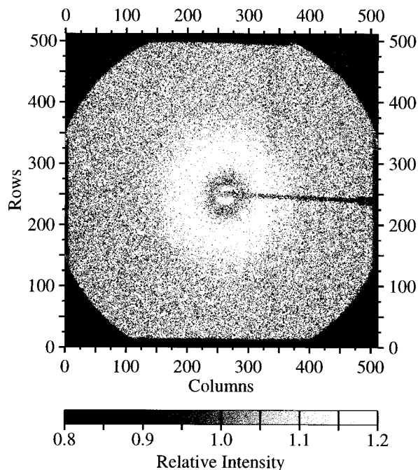
FIG. 7. The two-dimensional SAXS pattern right after inserting the gel-state suspension into the sample container ( T=0.5 h) divided by the scattering pattern measured at late times ( T=50 h). On the horizontal and vertical axis the number of the detector channel is depicted. The shadow of the beam stop is seen as the black stripe from the right to the center of the plot. A prominent feature is the presence of a ring, caused by nearest-neighbor correlations. The ring and other features are observed to have an almost perfect rotational symmetry and are independent of the sample orientation with respect to the incident x-ray beam.
