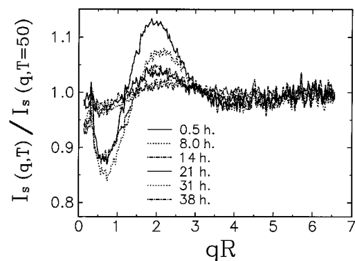
FIG. 8. Typical series of the integrated (one-dimensional) SAXS scattered intensity pattern after dividing the recorded patterns by the constant signal at T=50 h. Specifically at the region of the plateau of Fig. 2, which hardly shows any structure at first sight, the relative signal shows significant changes in the first few hours after inserting the suspension. This behavior slows down considerably towards T=50 h. The peak at qR=2.0 corresponds to the ring as shown in the two-dimensional patterns of Fig. 7. Note the drastic decrease in depth of the crest at qR=0.5 between T=14 h and T=21 h. Again the observations under different orientation of the sample container result in identical results.
