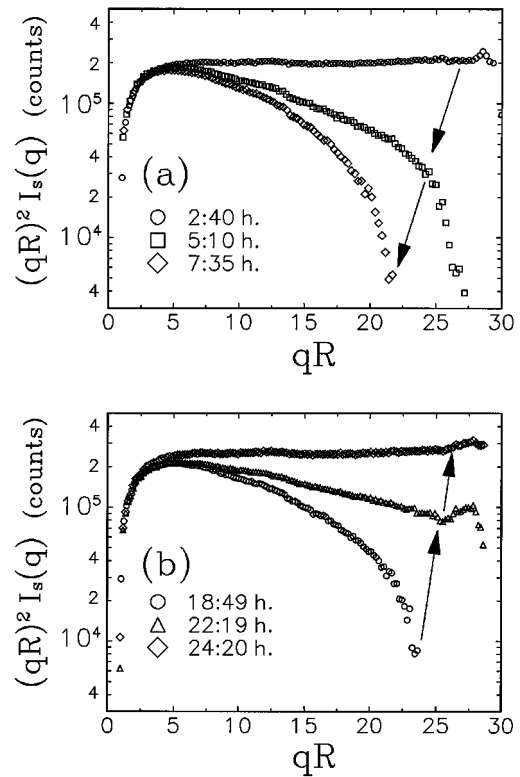
FIG. 5. Typical series of SAXS patterns of the colloidal suspension of disks as obtained at the Daresbury SRS. The suspension was inserted into the sample container from the sol state. In the legend the time after preparation is related to the symbols. The original SAXS patterns have been multiplied with (qR)^2 . First the pattern tends to decrease at the larger qR values, as shown in (a). After 10 h this process is reversed and the original signal is obtained after 40 h, as shown in (b). The tendency observed here is independent of the initial state before shear (sol or gel).
