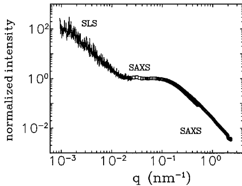
FIG. 1. Overview of the static scattered intensity I_s(q) as obtained from three scattering experiments. The smallest q regime, between 10^{-3} and 10^{-2} \text{nm}^{-1} , is captured by static light scattering (SLS). The intermediate q regime, between 10^{-2} and 10^{-1} \text{nm}^{-1} , and the largest q regime, between 10^{-1} and 10^0 \text{nm}^{-1} , are captured by small angle x-ray scattering (SAXS). The intensities displayed have been scaled to merge at the regions where the range in the scattering vector q overlaps.
