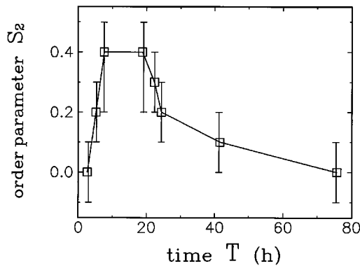
FIG. 6. Time dependence of the nematic order parameter S_2 characterizing the distribution function of the disk orientation, fitted to the data of Fig. 5. The positive value of S_2 indicates a preferential ordering of the colloidal disks as facing the container walls. The error bars on S_2 are mainly determined by background corrections, which become increasingly important at the large qR .
