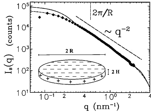
FIG. 2. Scattered intensity I_s(q) (diamonds) of a dilute, nongelating, suspension of disks in the range of the form factor. At large q , the intensity decays with q^{-2} (dashed line) as expected for randomly oriented thin disks. The solid curve is the calculated form factor of monodisperse thin disks with radius R = 12.5 \pm 0.5 nm and a thickness 2H = 1.0 \pm 0.1 nm. The dash-dotted curve is the calculated form factor of disks with the same dimensions with a Gaussian polydispersity in the radius of 4 nm. The colloidal disk is illustrated in the inset with its sizes and charge distribution.
