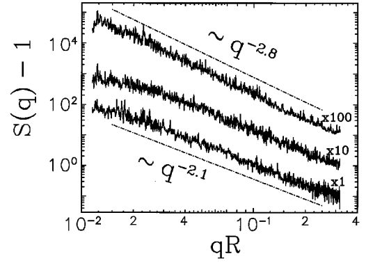
FIG. 4. Time series of the static structure factor S(q) - 1 vs qR as measured on the colloidal suspension of disks with a volume fraction \Phi_v = 0.0119 in water. At this volume fraction a strong gel is formed in 100 h. The patterns are plotted in the following order (from top to bottom); T = 2.5 h, 98 h, and 1.5 years. The patterns show an algebraic dependence, characterized by an exponent d that decays from d = 2.8 at T = 2.5 h to d = 2.1 at T = 1.5 years.
