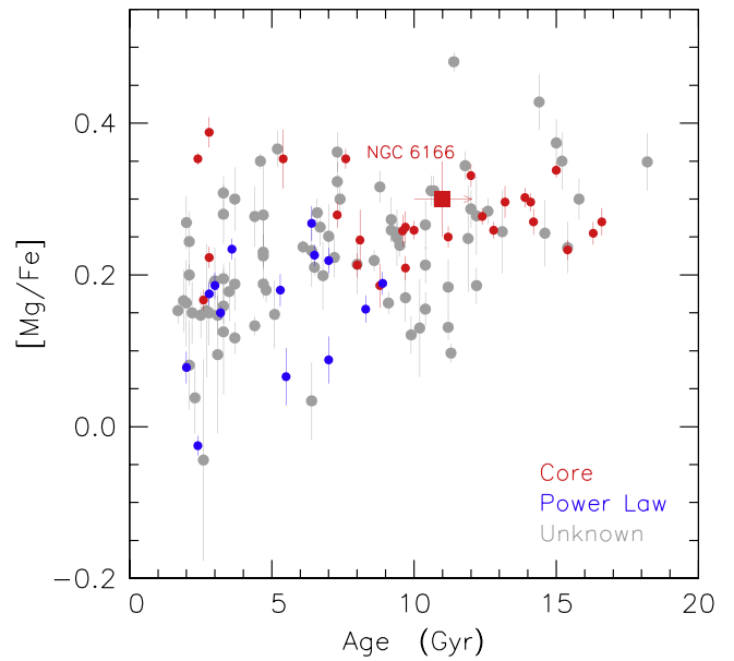
Figure 20. Correlation of [\text{Mg}/\text{Fe}] measure of \alpha element (over)abundance with stellar population age showing core-boxy-nonrotating galaxies in red, coreless-disky-rotating galaxies in blue, and galaxies with unknown type in gray. The metallicity and age measurements are from Thomas et al. (2005); the galaxy classifications are from Lauer et al. (2007) or from KFCB, and this figure is from KFCB with NGC 6166 added.
