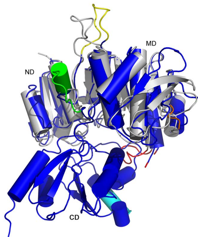
Figure 4. Comparison of crystal structures of full-length PaMpl and truncated NmMpl. The crystal structure of truncated NmMpl (grey, ND and MD only, PDB id 3eag) is similar to PaMpl (blue) and can be superimposed with an r.m.s.d. of 2.2 Å over 311 C \alpha atoms with a sequence identity of 57%. The main differences are: NmMpl lacks the PaMpl -specific sequence segments 141–152 (green), 262–285 (orange) and 444–450 (cyan); NmMpl residues 152–163 are positioned differently compared to the corresponding residues 161–171 in PaMpl (yellow); and the segment corresponding to a loop (residues 199–208, red) in NmMpl is disordered in PaMpl (residues 210–215, flanking residues 209 and 216 are in red). doi:10.1371/journal.pone.0017624.g004
