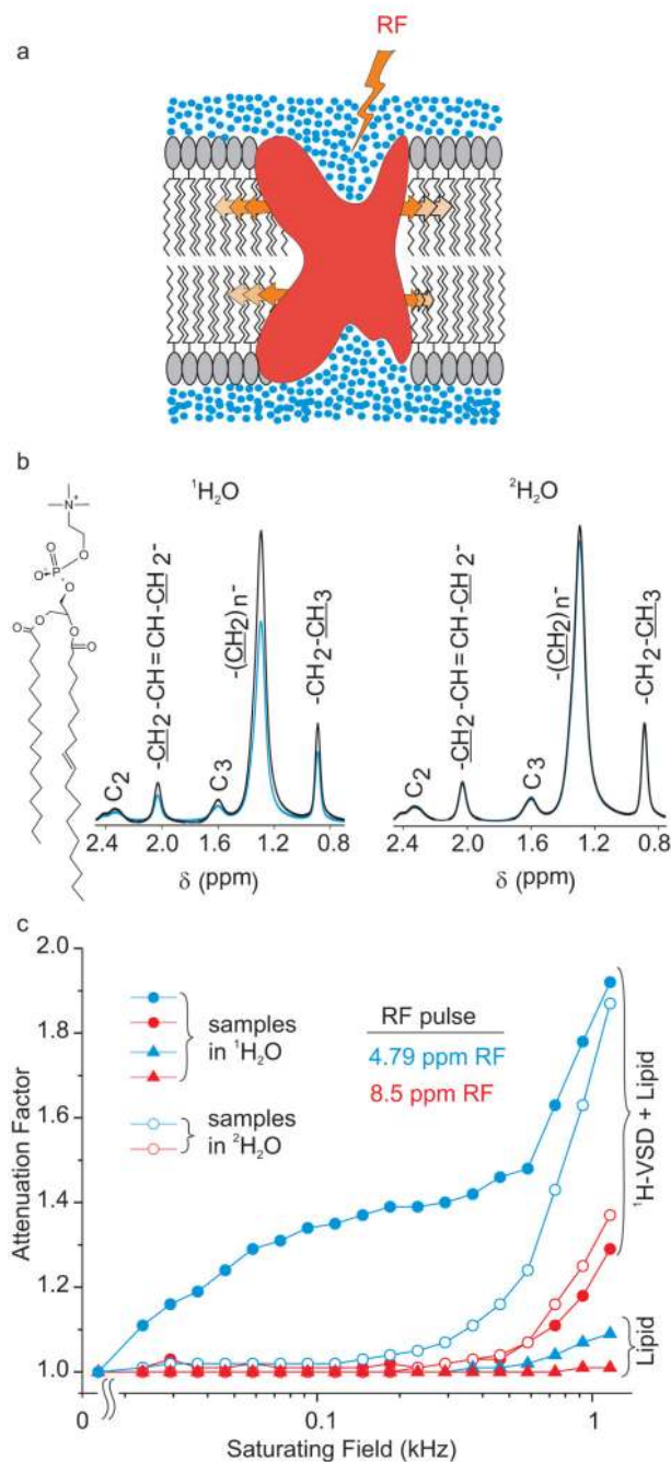
Figure 4. Interaction of water and S1–S4 voltage-sensing domains within lipid membranes a) Schematic representation of crevices in S1–S4 voltage-sensing domains (red) filled with water (blue) and an experiment in which selective, saturating radio frequency (RF) pulses were applied at the water resonance (4.792 ppm). Magnetization transfer from water through protein to the surrounding lipid results in the attenuation of the lipid ^1\text{H} NMR signals. b) Aliphatic region of MAS ^1\text{H} NMR spectra of a lipid sample containing S1–S4 voltage-sensing domains in the presence of ^1\text{H}_2\text{O} (left spectrum) or ^2\text{H}_2\text{O} (right spectrum). Lipid resonances for both POPC and POPG (present in a 1:1 mix) are indicated on the spectra,
