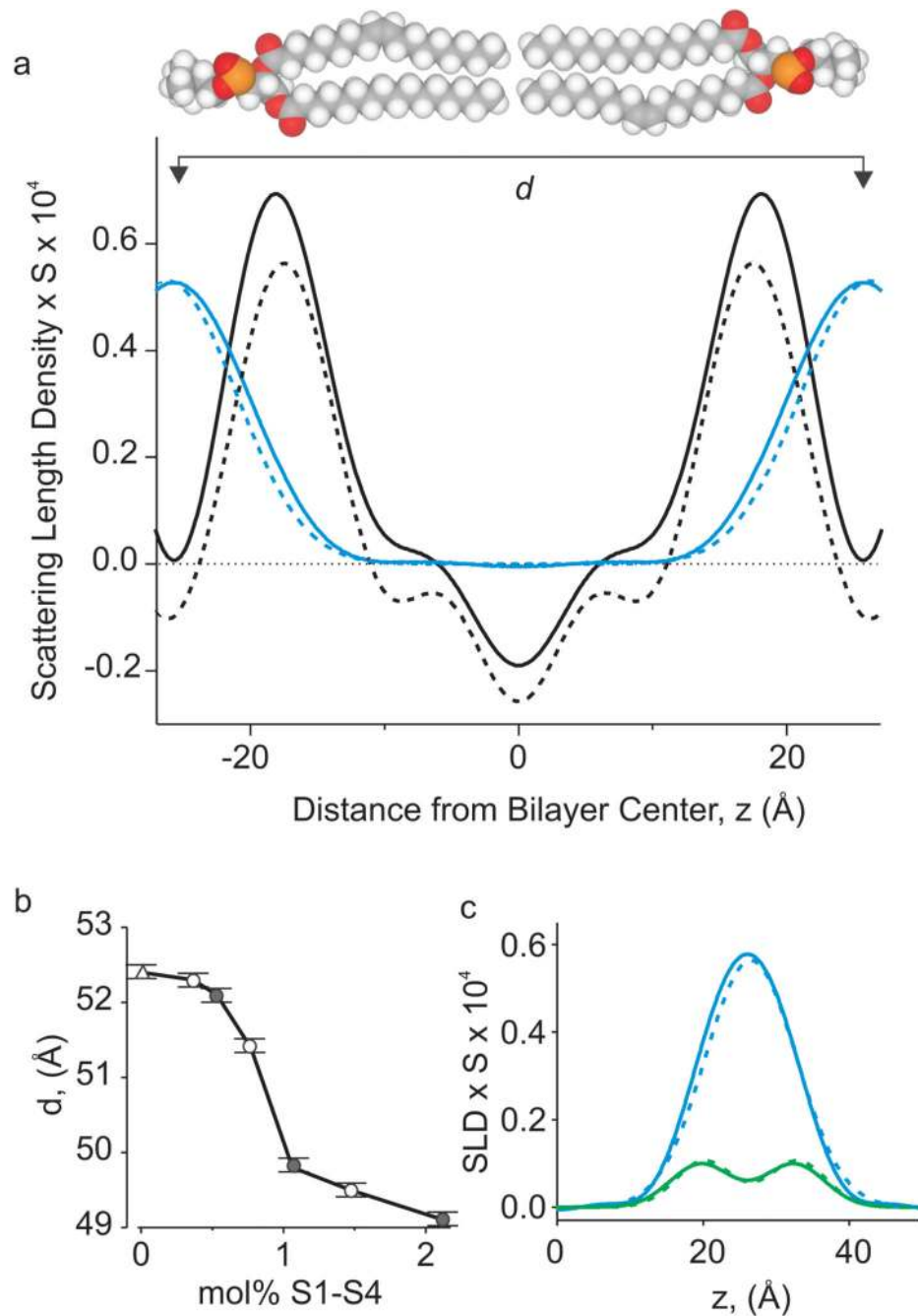
Figure 2. Scattering length density profiles for bilayers containing S1-S4 voltage-sensing domains
