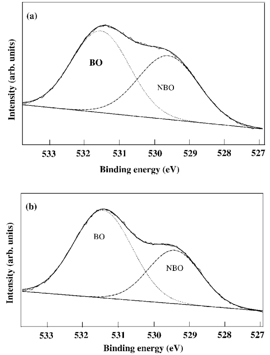
Fig. 8. The resulting fit (—) from the BO and NBO peaks (---) to the high-resolution O 1s spectra for (a) x = 0.075 and (b) x = 0.026 fractured glass samples.
