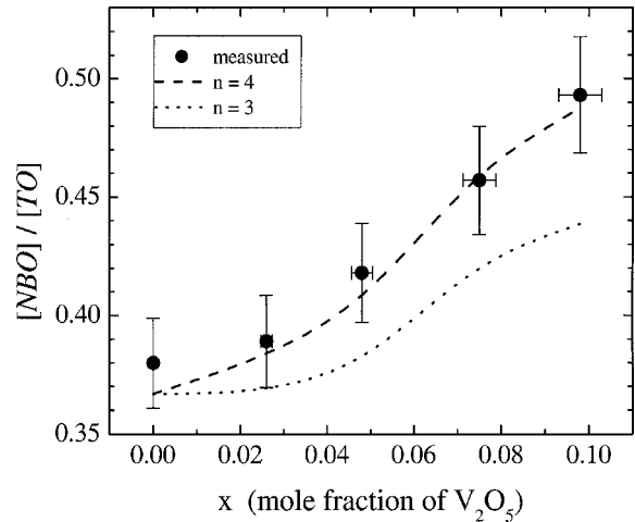
Fig. 9. Comparison of measured [NBO]/[TO] ratios as a function of V_2O_5 content to ratios calculated from Eq. (1) for different values of n .
