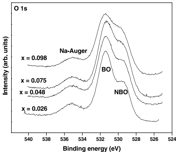
Fig. 3. High-resolution O 1s core level spectra for the V_2O_5 sodium silicate glass samples.
