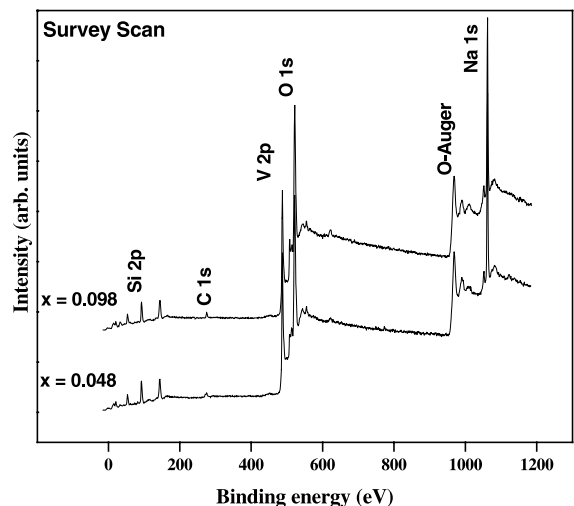
Fig. 1. XPS survey scans of two fractured vanadium sodium silicate glasses.
