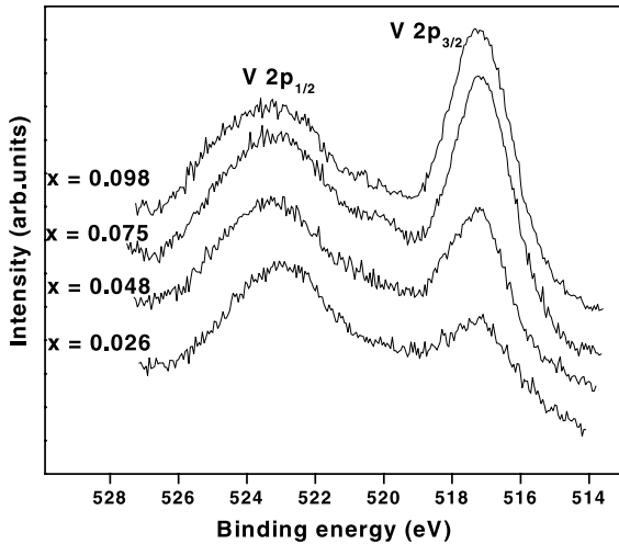
Fig. 2. High-resolution core level spectra of the V 2p transition for fractured glass samples with varying V_2O_5 content.
