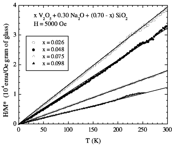
Fig. 6. The inverse of the magnetic susceptibility H/M^* as a function of the temperature for (V_2O_5)_x(Na_2O)_{0.30}(SiO_2)_{0.70-x} glass samples. The solid lines represent fits to a Curie temperature-dependent behavior.
