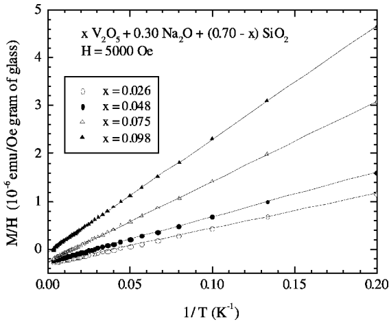
Fig. 5. The magnetic susceptibility M/H as a function of the inverse temperature 1/T for (V_2O_5)_x(Na_2O)_{0.30}(SiO_2)_{0.70-x} glass samples. The solid lines are the high-temperature extrapolations for determining (M/H)_{\text{constant}} .
