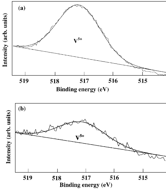
Fig. 7. The resulting fit (—) to the high-resolution V 2p_{3/2} spectra for (a) x = 0.098 and (b) x = 0.048 fractured glass samples.
