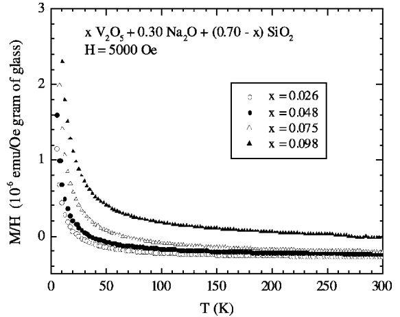
Fig. 4. The magnetic susceptibility M/H as a function of temperature T for the (V_2O_5)_x(Na_2O)_{0.30}(SiO_2)_{0.70-x} glass samples.
