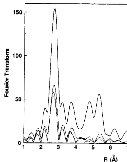
Figure 2. Magnitude of the Fourier transform ( k^3 -weighted, \Delta k = 2.6 – 13.5 \text{ \AA}^{-1} ) of Ir powder (solid line), Ir n /MgO (dot-dashed line), Ir 6 /MgO (dot-dot-dashed line), and Ir 4 /MgO (dotted line).
