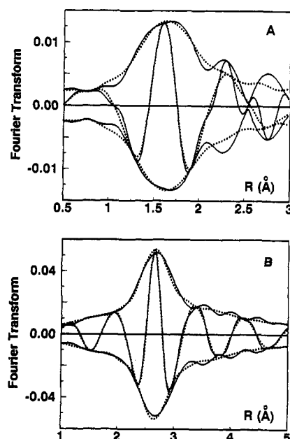
Figure 8. (A) Fourier transform ( k^3 -weighted, \Delta k = 3.5 – 12.5 \text{ \AA}^{-1} , Ir-Mg phase-corrected) of difference file (isolated EXAFS minus calculated Ir-Ir(1) + Ir-O(1)) (solid line) and calculated Ir-Mg EXAFS function (dotted line) for Ir 4 /MgO. (B) Fourier transform ( k^3 -weighted, \Delta k = 3.5 – 12.5 \text{ \AA}^{-1} , Ir-O phase-corrected) of difference file (isolated EXAFS minus calculated Ir-Ir(1) + Ir-Mg) (solid line) and calculated Ir-O(1) EXAFS function (dotted line) for Ir 4 /MgO.
