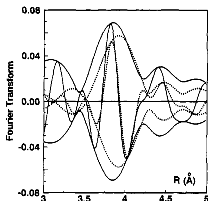
Figure 7. Fourier transform ( k^3 -weighted, \Delta k = 3.5 – 12.5 \text{ \AA}^{-1} , Ir-Ir phase- and amplitude-corrected) of the difference file (isolated EXAFS minus calculated Ir-Ir(1) + Ir-O(1) + Ir-Mg) (solid line) and calculated Ir-Ir(2) EXAFS function (dotted line) for Ir 4 /MgO (notation in Table I).
