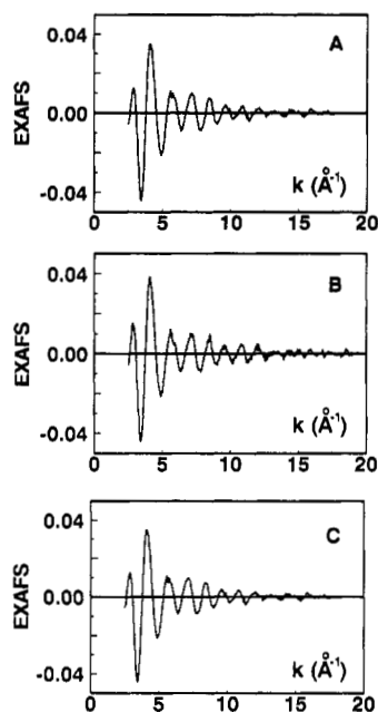
Figure 1. Raw EXAFS data characterizing (A) Ir 4 /MgO, (B) Ir n /MgO, and (C) Ir 6 /MgO.
