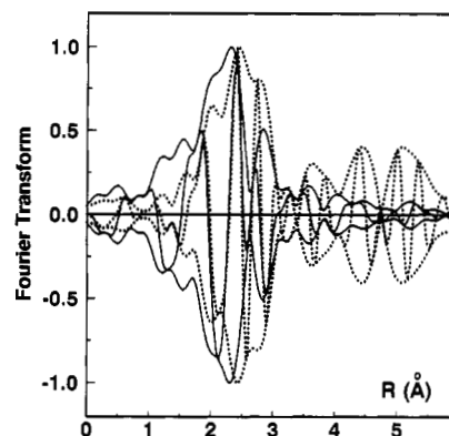
Figure 3. Magnitude (envelope) and imaginary part (oscillations within envelope) of Fourier transform ( k^1 -weighted, \Delta k = 2.6 – 13.5 \text{ \AA}^{-1} ) of EXAFS function characterizing Ir 4 /MgO (solid line) and Ir powder (dotted line). Data are scaled to facilitate the comparison.
