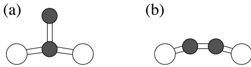
FIG. 5. Possible bonding configurations for an extra oxygen atom in a\text{-SiO}_2 . (a) ‘‘Threefold’’ configuration in which an extra oxygen binds to a bridge-bonded oxygen. (b) ‘‘Peroxyl bridge’’ configuration in which an extra oxygen inserts into a bridge bond. Filled and open circles represent oxygen and silicon atoms, respectively.
