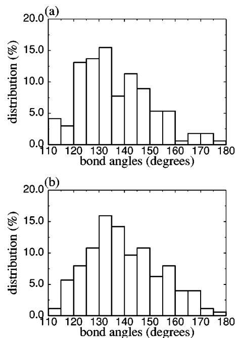
FIG. 4. Histograms of Si–O–Si bond angles, for bond angles located (a) within 5 Å of the interface, and (b) between 5 and 10 Å from the interface.
