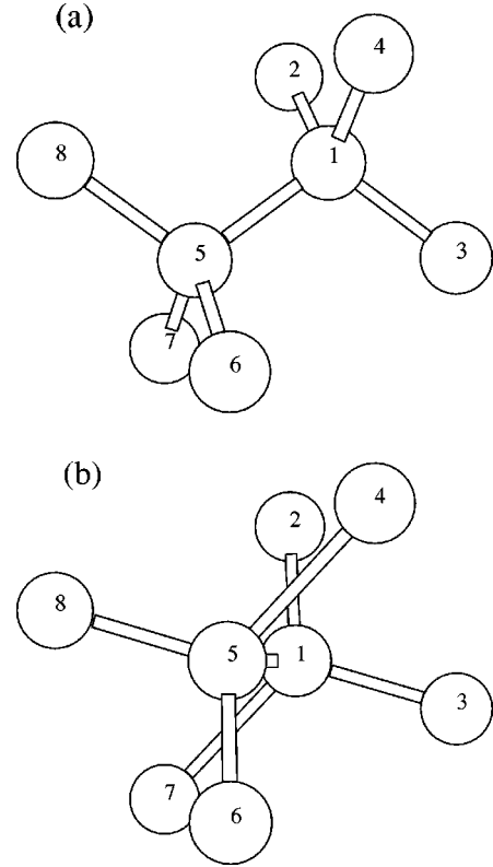
FIG. 1. The WWW bond-switching move (Ref. 28) used in the Monte Carlo simulations. (a) Initial configuration. Atoms 1 and 4 are first neighbors, and atoms 1 and 7 are second neighbors. (b) After bond switch. Atoms 1 and 7 are now first neighbors, while atoms 1 and 4 are second neighbors.
