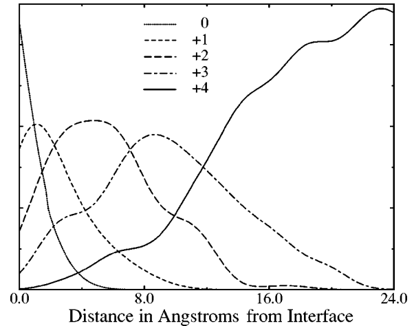
FIG. 2. Oxidation number of Si versus distance of Si from interface, as obtained from the Monte Carlo simulations. Curves represent distribution profiles for five different oxidation states, smoothed by a Gaussian broadening of width \sim 2 Å. Data is compiled from six different structures with a total of \sim 10^3 Si atoms.
