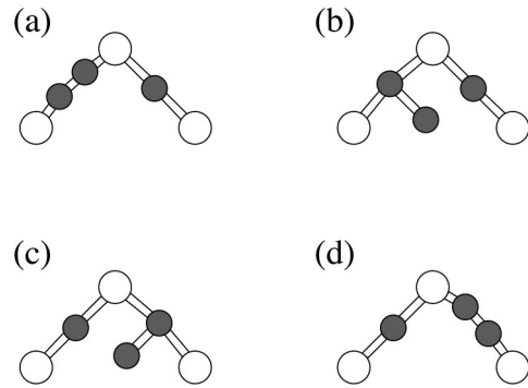
FIG. 6. Proposed mechanism for diffusion of atomic oxygen in a\text{-SiO}_2 . (a) Initial configuration with peroxyl bridge at left. (b) Peroxyl bridge excites into a threefold structure. (c) Extra oxygen atom jumps to a neighboring bond. (d) Threefold structure decays to form new peroxyl bridge at right.
