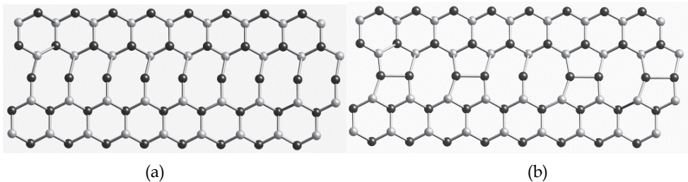
Fig. 1. Models of the core structure of an unreconstructed (a) and a reconstructed 30° partial dislocation (b) according to Northrup et al. (1981) and Marklund (1983).
