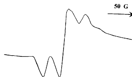
Fig. 7. EPR spectrum of the deposited mixture xenon–heptane–Freon-113 (400:1:2) irradiated with fast electrons (40 kGy) at 15 K.
