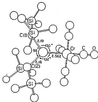
Fig. 12. Crystal structure of [(\text{Me}_3\text{Si})_2\text{CH}]_2\text{Sn}-\text{Cr}(\text{CO})_5 (45). Reprinted with permission from J. Chem. Soc., Chem. Commun. 1974, 893. Copyright by The Chemical Society
