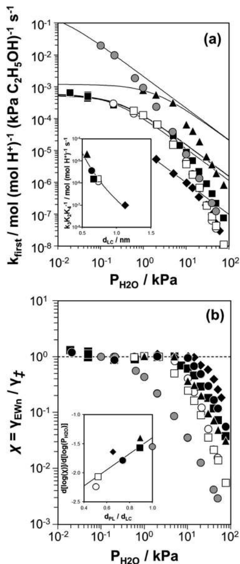
Fig. 7 (a) Apparent first-order bimolecular ethanol dehydration rate constant (per \text{H}^+ , 373 K) and (b) activity coefficient ratio ( \chi = \gamma_{\text{EW}_n} / \gamma_{\#} ) from eqn (7), as a function of \text{H}_2\text{O} pressure on H-Al-Beta-F(2.0) (■), H-Al-TON (▲), H-Al-FAU (◆), H-Al-MFI (●), H-Al-AEI (□), H-Al-CHA (○), and HPW/Si-MCM-41 (●). Solid lines in (a) reflect regression of measured rate constants to eqn (7). Inset (a): dependence of k_3K_2K_4^{-1} values on the largest included sphere diameter of zeolite pores ( d_{\text{LC}} ). Inset (b): slopes of the data sets in (b) in the high water pressure limit, as a function of the channel undulation parameter ( d_{\text{PL}}/d_{\text{LC}} ). Solid lines in both insets are to guide the eye.
