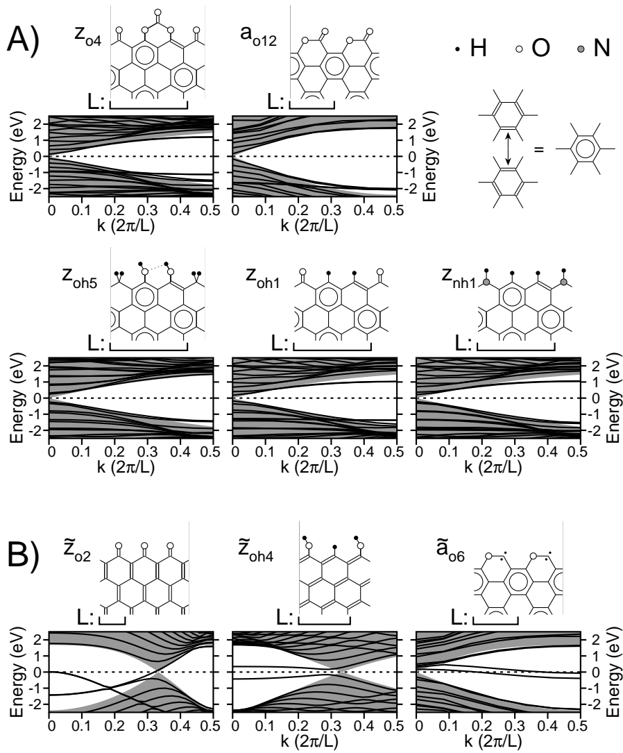
FIG. 5: A) Scheme and electronic band-structure of the five most stable oxygen-, water- and ammonia-terminated edges of a graphene nanoribbon. Carbon-carbon bonds are represented with the standard notation, while hydrogen, oxygen and nitrogen atoms are the small circles. The structures are periodic along the ribbon-edge with periodicity L . The gray area corresponds to the electronic-bands allowed in “bulk” graphene. The dashed line is the Fermi level. The top-right inset displays the standard representation of the aromatic carbon ring. B) Three examples of “metallic/magnetic” edges (see the definition in the text). \tilde{z}_{o2} , non-magnetic within DFT-GGA calculations, is found to be magnetic when hybrid DFT functionals are used 27 ; \tilde{z}_{oh4} and \tilde{a}_{o6} both magnetic. The \tilde{a}_{o6} structure is non-aromatic according to our definition, since the two small dots represent a diradical, which is the only representation compatible with the carbon chemical valence.
