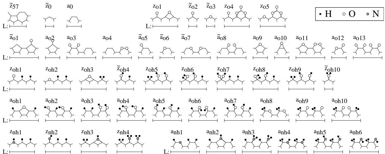
FIG. 1: Scheme and labelling of the oxygen- (right top line and second line from top), water- (third and fourth lines from top), and ammonia-terminated (bottom line) edges of a graphene nanoribbon considered in this work. Hydrogen, oxygen and nitrogen atoms are the small circles, while carbon atoms are not explicitly represented; dashed lines indicate hydrogen bonds. The structures are periodic along the ribbon-edge with periodicity L , and are ordered with respect to increasing O and N density and, at equal density, to increasing formation energy. A tilde over an edge label indicates that that structure is not an aromatic one.
