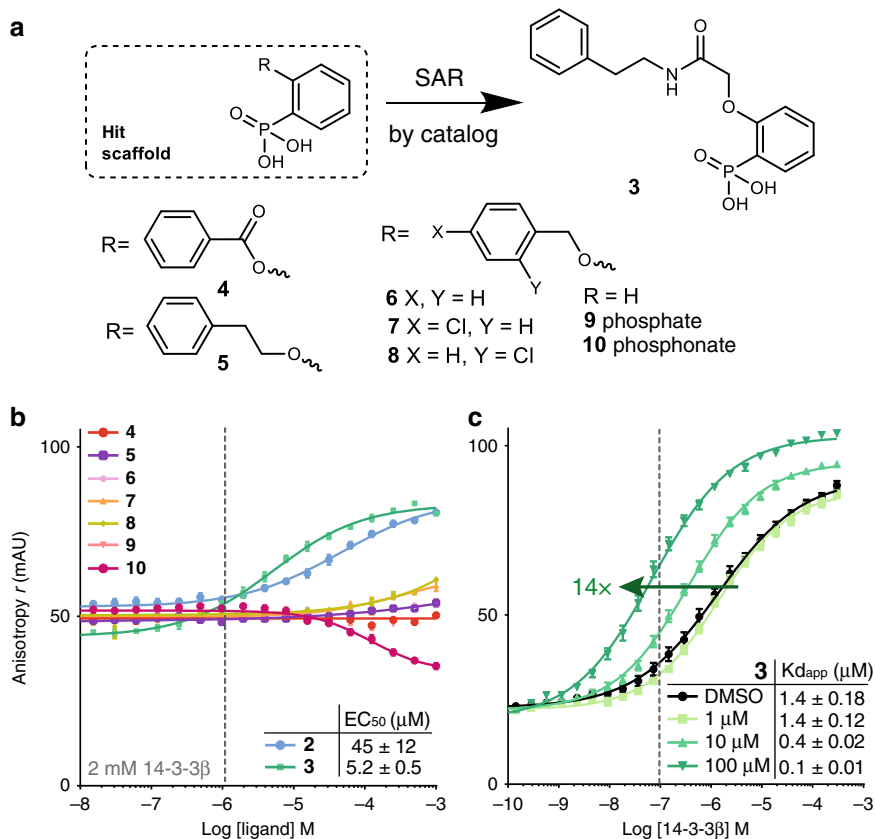
Fig. 2 Initial optimization via SAR-by-catalog of the hit scaffold 2 -based series. a Eight derivatives of 2 were selected for molecular docking and in vitro testing. Titration curves of b ligands on 2 μM 14-3-3β and 100 nM fluorescently-labeled ChREBP peptide, and c of 14-3-3β on 100 nM fluorescently-labeled ChREBP peptide in presence of increasing concentrations (1, 10, 100 μM) of compound 3 . Data and error bars represent mean ± SEM, n = 3 replicates. Source data are provided as a Source data file.
