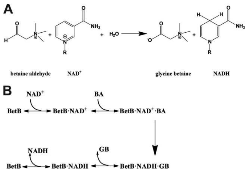
FIG 1 Reaction catalyzed by S. aureus BetB and proposed mechanism. (A) NAD + -dependent oxidation of betaine aldehyde to glycine betaine. (B) Ordered Bi Bi mechanism proposed for BetB.
