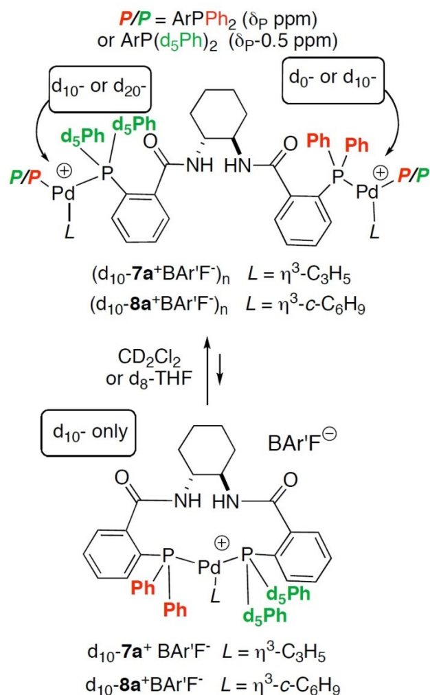
Figure 3. Use of isotopically desymmetrized ligand ( R,R )- d 10 - 1a to distinguish monomeric ( n = 1) from oligomeric ( n > 1) forms of Pd complexes ( d 10 - 7a + BAR' F − ) n and ( d 10 - 8a + BAR' F − ) n via 31 P 31 PCOSY.
