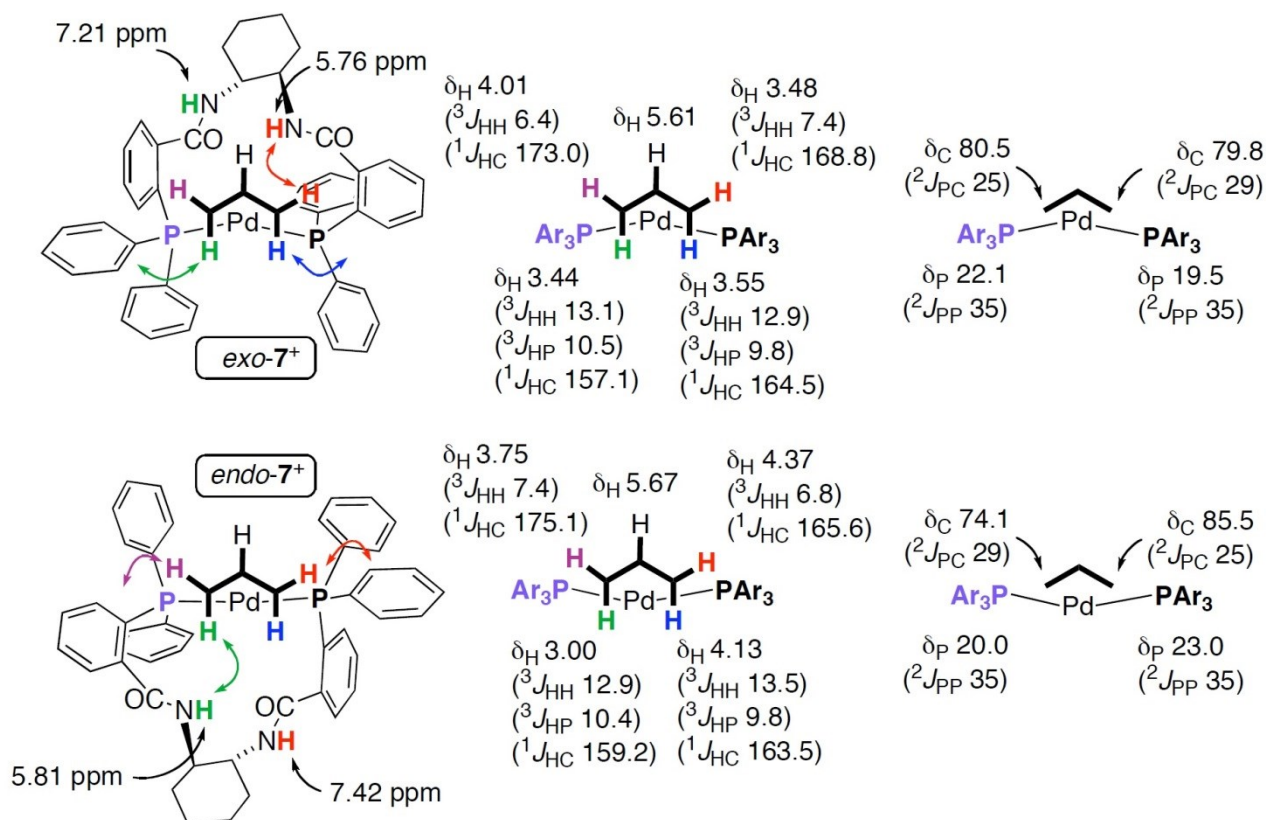
Figure 4. Color-coding showing the static P,P -Pd- \eta^3 -allyl unit during interconversion ( k = 2.6(\pm 0.3) \text{ s}^{-1} , \text{CD}_2\text{Cl}_2 , 25 °C) of monomeric exo\text{-}7^+ and endo\text{-}7^+ with selected NMR data ( \delta/\text{ppm} , J/\text{Hz} ) and nOe contacts.
