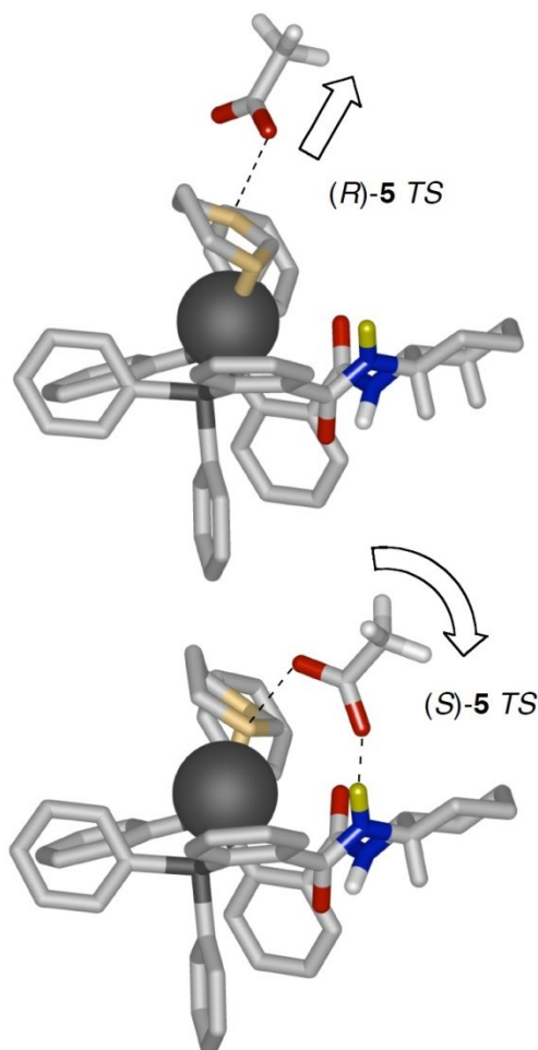
Figure 9. ‘Side view’ of DFT-optimized TS structures leading to exo-8 + via ionization of mismatched cyclohexenyl acetate ( R )- 5 (upper) and matched cyclohexenyl acetate ( S )- 5 (lower). The approximate motions of the acetate groups leading to ionization are indicated with arrows.
