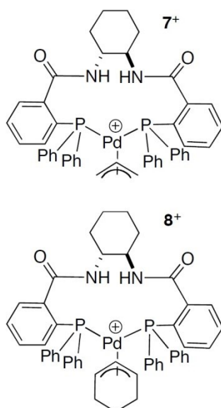
Chart 2. Cationic Monomeric Palladium \eta^3 -Allyl ( 7 + ) and \eta^3 -Cyclohexenyl ( 8 + ) Complexes of the Standard Ligand ( R,R )- 1 Generated in situ from Oligomer, then Studied by NMR.
