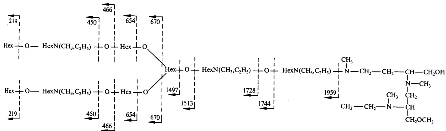
Scheme 3. Sequence information from the EI mass spectrum (60 eV) of N -acetylated, permethylated and reduced Galp- \beta (1 \rightarrow 4)-GlcNAc \rho - \beta (1 \rightarrow 2)-Manp- \alpha (1 \rightarrow 3)-[Galp- \beta (1 \rightarrow 4)-GlcNAc \rho - \beta (1 \rightarrow 2)-Manp- \alpha (1 \rightarrow 6)-]Manp- \beta (1 \rightarrow 4)-GlcNAc \rho -(1 \rightarrow 4)-GlcNAc \rho - \beta (1 \rightarrow N)-(Ser)-Asn.
