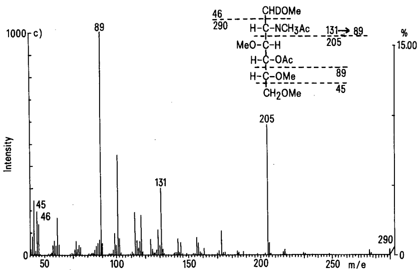
Figure 4. EI mass spectra (70 eV) of the partially methylated alditol acetates of (a) 1,5-di- O -acetyl-2,3,4,6-tetra- O -methyl-mannitol-1- 2 H 1 , (b) 1,3,5-tri- O -acetyl-2,4,6-tri- O -methyl-mannitol-1- 2 H 1 , and (c) 4-mono- O -acetyl-1,3,5,6-tetra- O -methyl-2- N -methyl-acetamido-2-deoxy-glucitol-1- 2 H 1 .
