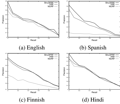
Figure 2: Precision-Recall Curve
