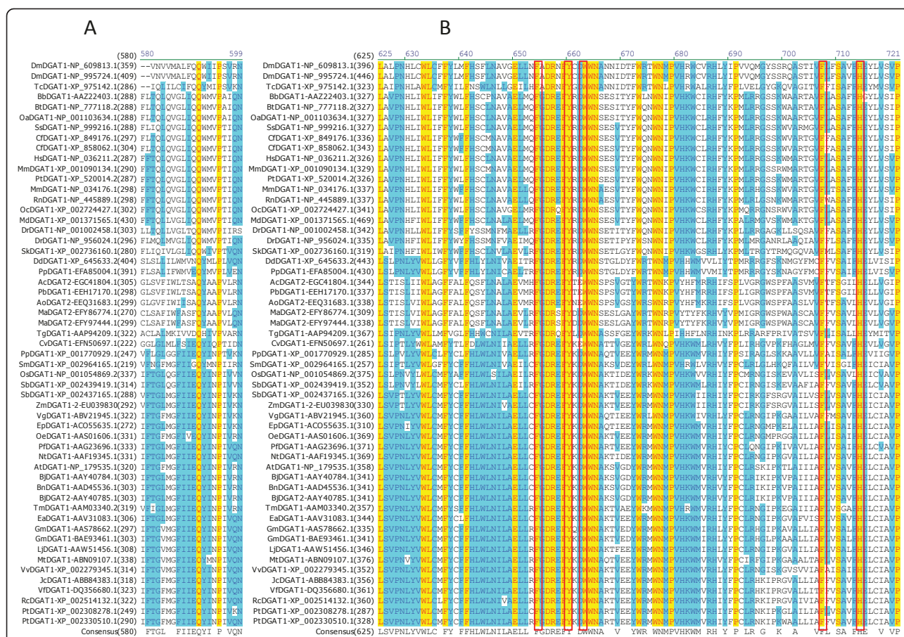
Figure 4 Identification of completely conserved amino acid residues in sequence motifs 4-5 of DGAT1s. (A) DGAT1-Motif 4 (QP Block), (B) DGAT1-Motif 5 (LWLFEEFDRFYWWNWWNPPFSHP Block); The first boxed F residues are also conserved in DGAT2s; The boxed Y, W and the second F residues are mutated in TmdGAT1 and the boxed H residue is mutated in MmdGAT1). Refer to Figure 3 legend for additional information.
