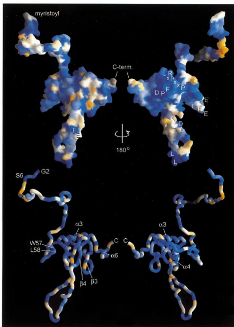
Fig. 2. Sequence conservation superimposed onto the surface and the backbone structure of HIV-1 Nef. The colour coding corresponds to the degree of conservation ranging from 30% (orange) to 84% (white, average conservation) to 100% (blue). Some of the interaction sites listed in Table I are indicated on the structure. The figure was generated with GRASP (Nicholls et al. , 1991).
