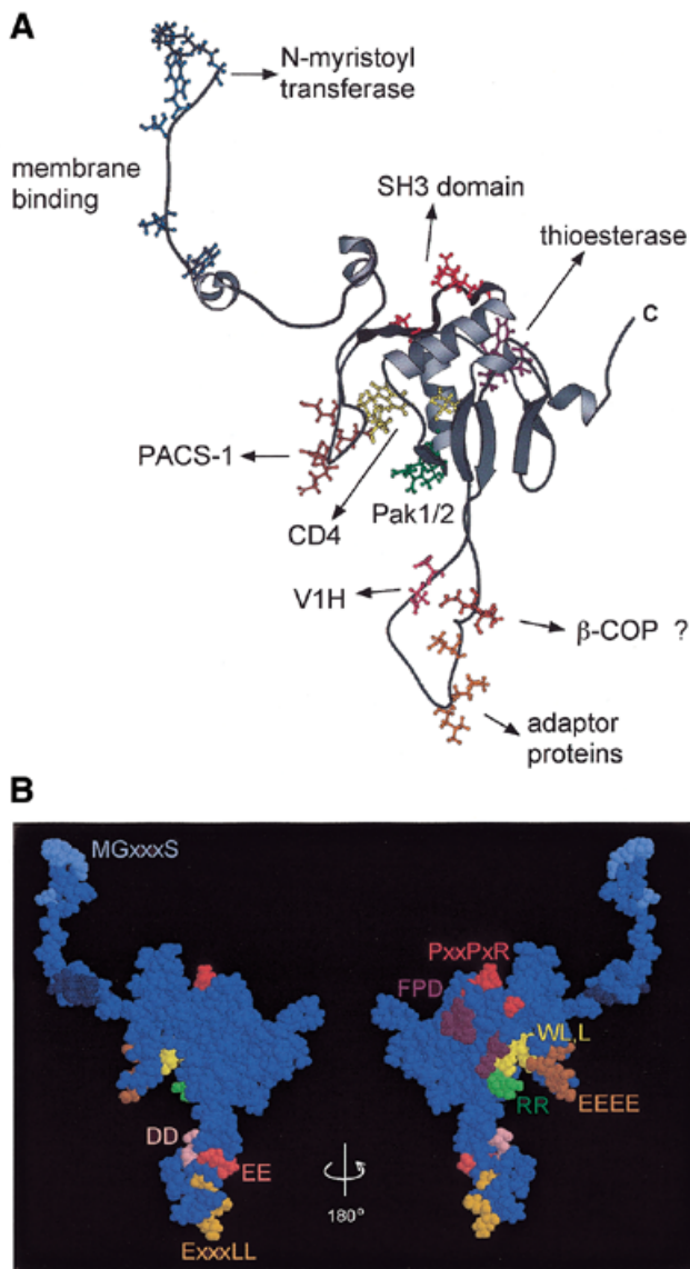
Fig. 1. Location of functional motifs in the HIV-1 Nef structure. (A) Functional motifs in HIV-1 Nef (Table II) and their location in the full-length structure as derived from the NMR structure assembly. Binding sites for the known interacting proteins are indicated. (B) The van der Waals surface presentation of Nef indicates the accessibility of the interacting residues. The colour coding corresponds to the labelled residues in (A).
