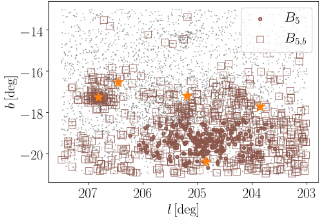
Fig. 8. Top panel: sky distribution of the sources belonging to group B_{5,b} (brown empty squares), group B_5 (brown dots), and all the sources in the Belt region defined in the text (grey dots). The orange stars mark the position of \sigma Ori, \zeta Ori, \epsilon Ori, \eta Ori, and \delta Ori. Bottom panels: distribution in 3D galactic co-ordinates of group B_{5,b} (brown squares), and of all the sources belonging to the Belt region (grey dots).
