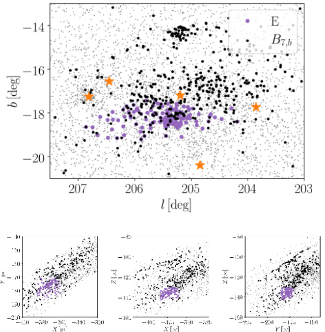
Fig. 10. Distribution in the sky ( top ) and in 3D space ( bottom ) of the stars belonging to group B_{7,b} (black dots) compared to those in group E (purple dots). The grey dots represent all the sources in the Belt region. The orange stars are the same as defined in Fig. 7.
