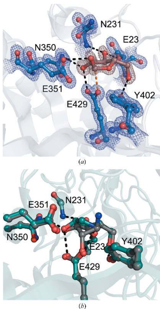
Figure 3 Active site and conformational itinerary of MgGH51 . ( a ) Active-site arrangement of MgGH51 around \alpha -L-arabinofuranose. Active-site residues interacting with \alpha -L-arabinofuranose (brown) are shown as blue sticks. Apparent hydrogen-bonding interactions are shown as black dashed lines. The interaction between the catalytic nucleophile and the anomeric C atom is shown as an orange dashed line. Electron density is shown as a mesh contoured at 1.5\sigma . ( b ) Overlay of the AraDNJ and \alpha -L-AraAZI ligands within the MgGH51 active site. The active-site residues and ligand from the \alpha -L-AraAZI complex are shown as grey sticks. The active-site residues and ligand from the AraDNJ complex are shown as cyan sticks. Apparent hydrogen-bonding interactions are shown as black dashes.
