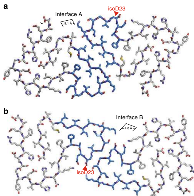
Fig. 5 Model of A \beta^{20-34} , isoAsp ^{23} as the core of an A \beta^{1-42} modified polymorph. a Model of A \beta^{1-42} , isoAsp ^{23} centered on interface A. b Centered on interface B. Blue residues correspond to the crystal structure core (A \beta^{20-34} , isoAsp ^{23} ), gray sticks correspond to the modeled extension (1-19 and 35-42)
