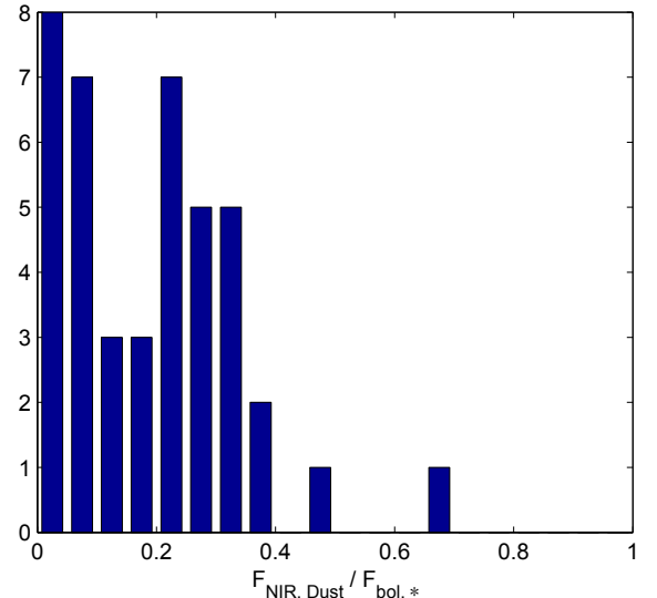
Fig. 18. Histogram of the fraction f_{\text{rep}} of stellar bolometric luminosity reprocessed to near infrared for non-binary objects.
