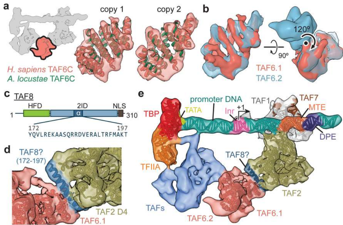
Figure 4. Structural TAFs within lobe C
