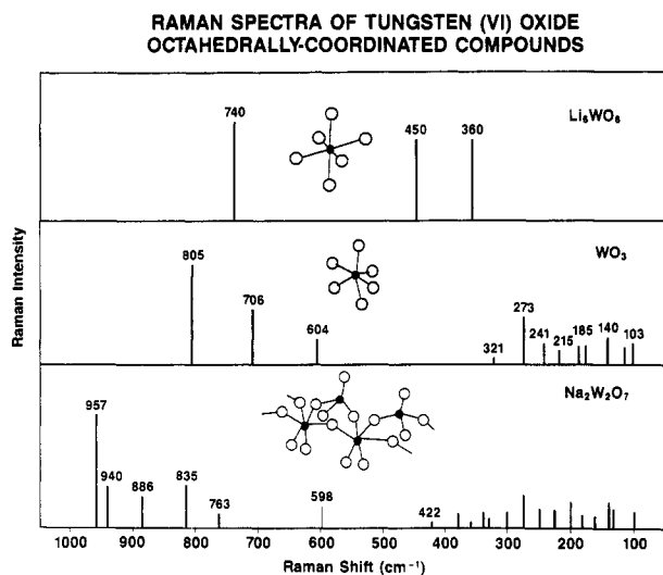
Figure 5. Schematic laser Raman spectra of compounds possessing WO 6 groups: Li 6 WO 6 , WO 3 , and Na 2 W 2 O 7 .
