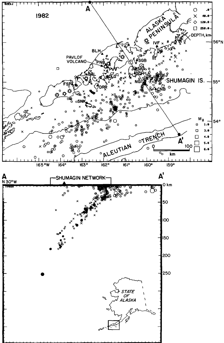
Fig. 1. Seismicity recorded by the Shumagin seismic network in eastern Aleutians, Alaska, during 1982. The location of this map in the eastern Aleutians is indicated in the lower right-hand corner of the cross section. (Top) Map view showing epicenters where symbol type is keyed to depth and symbol size is keyed to magnitude. Seismic stations are designated by a solid triangle and a three-letter code. Stations BLH, PVV, SGB, SAS, and CNB are equipped with three-component seismometers. Active volcanoes on the Alaska Peninsula are shown as marked open circles. (Bottom) Depth cross section with no vertical exaggeration taken along the profile A-A'. The solid circles represent the hypocenters of the 15 earthquakes relocated in this study.
