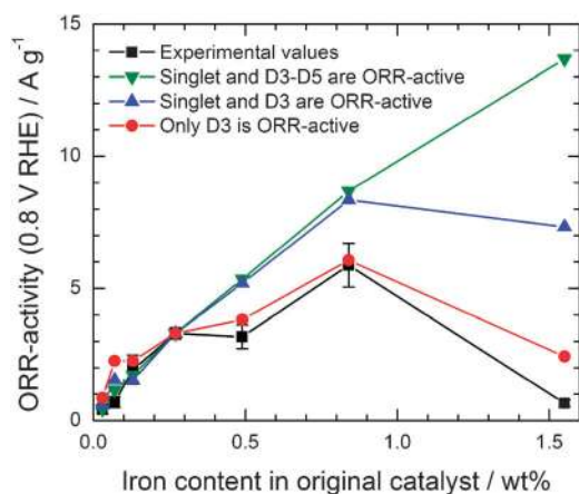
Fig. 8 Comparison between experimental ORR activities reproduced from Fig. 4a (black squares) and calculated ORR activities according to three hypotheses: (1) iron nitride nanoparticles (D4 and D5), the singlet and D3 ( \text{N-FeN}_{2+2} \cdot \cdot \cdot \text{N}_{\text{prot}}/\text{C} composite sites) are all ORR active (green triangles); (2) the singlet and D3 are both active (blue triangles); (3) only D3-sites are ORR active (red circles).
