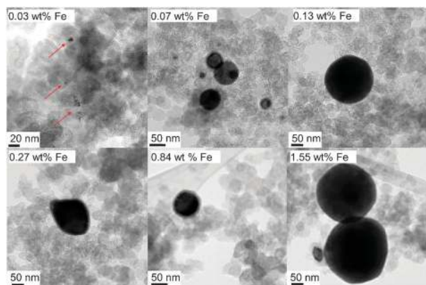
Fig. 3 TEM images of the quasi-spherical particles of iron nitride observed in all the catalysts prepared in this study, with each catalyst's iron content specified in the label.
