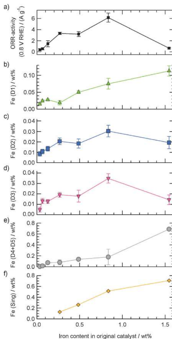
Fig. 4 Compared evolution of the catalysts' ORR-activity and the relative composition of each Fe-species with the bulk iron content.
