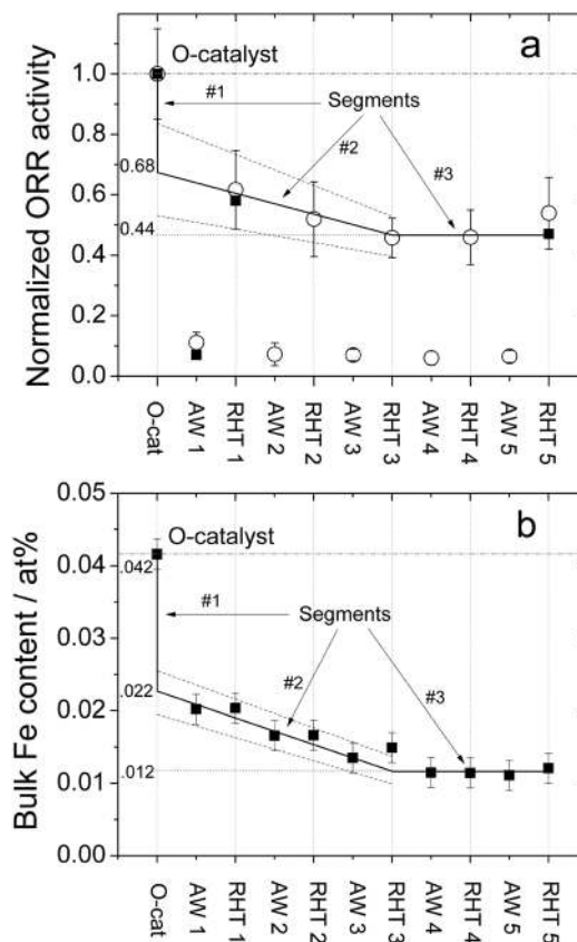
Fig. 6 Activity recovered by reheat-treatment in argon of the acid-washed catalyst of ref. 28, having a similar Fe content (0.20 wt% Fe) than the catalyst used in Fig. 4a (0.27 wt% Fe). (a) Normalized activity, based on that of the original catalyst (Ocat), as measured in RDE (open circles) or PEM fuel cell (filled squares) at various steps of five successive acid washing/reheat-treatment cycles. Acid washed and reheat-treated catalysts are labeled AW x and RHT x , respectively, x denoting the cycle number. (b) Bulk Fe content at each step of the five acid washing/reheat-treatment cycles described in (a), as measured by neutron activation analysis.
