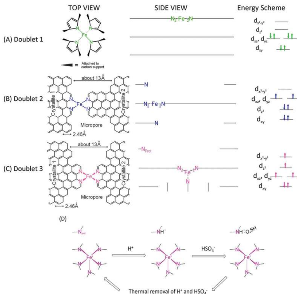
Fig. 2 Side views and top views of the proposed structures of: (A) the \text{FeN}_4/\text{C} catalytic site in heat-treated, macrocycle-based catalysts assigned to Mössbauer doublet D1, (B) the \text{FeN}_{2+2} -like micropore-hosted site found in the catalyst prepared with iron acetate and heat-treated in ammonia assigned to doublet D2, and (C) the \text{N-FeN}_{2+2} -like composite site, where \text{N-FeN}_{2+2} is assigned to doublet D3. In all side views, graphene planes are drawn as lines. In (B), the distance between the two nitrogen atoms belonging to the graphene planes above and below the \text{FeN}_{2+2} -plane is similar to that in crystalline iron phthalocyanine (see Fig. S1, ESI†), thus similarly influencing the lattice contribution to the quadrupole splitting. In (C), the iron(II) ion in \text{N-FeN}_{2+2} is coordinated by five pyridinic nitrogen atoms, one of them belonging to a plane located at the vertical below the \text{N}_4 -plane. This axial nitrogen coordination moves the iron(II) ion out of the \text{N}_4 -plane towards the fifth coordinating nitrogen atom. Doublet 3 may exist as \text{N-FeN}_{2+2}/\text{C} or as a composite site \text{N-FeN}_{2+2} \cdot \text{N}_{\text{prot}}/\text{C} , where \text{N}_{\text{prot}} is a protonable pyridinic nitrogen atom appearing at the edge of the upper plane in the side view of D3. 28 \text{N}_{\text{prot}} is too far from \text{N-FeN}_{2+2} to have an influence on the Mössbauer spectrum of D3, but it is close enough to drastically improve the turn-over frequency of the composite site proposed in (C). Fig. 2 also shows the energy schemes of D1, D2, and D3, as well as the filling of the molecular orbitals for the iron(II) ion in the structure proposed for each site according to its proposed spin state: low in D1, intermediate in D2, and high in D3. 47 Part (D) of Fig. 2 schematizes the changing ORR-activity of the composite \text{N-FeN}_{2+2} \cdot \text{N}_{\text{prot}}/\text{C} site, where \text{N-FeN}_{2+2}/\text{C} has the D3 signature; the activity of the composite site is low when the basic N-group neighbouring the \text{N-FeN}_{2+2}/\text{C} moiety is unprotonated (left) or protonated and anion-neutralized (right). The activity is high when this N-functionality is protonated but not neutralized (center). 28
