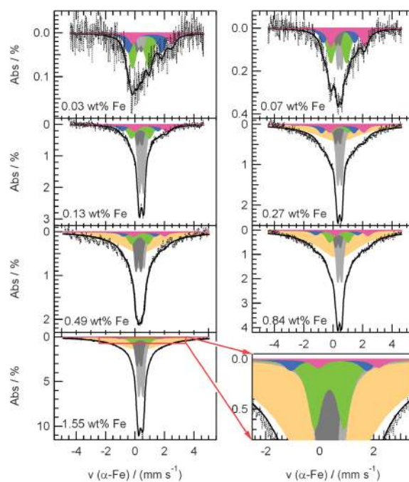
Fig. 1 Deconvoluted Mössbauer spectra of the Fe/N/C-catalysts. The iron content of the original catalyst is given as an inset in each spectrum.
