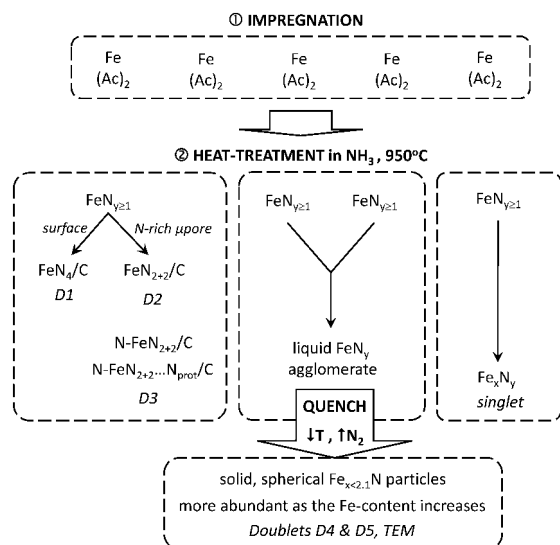
Fig. 9 Scheme of the model proposed for the formation of the various Fe-species present in the Fe/N/C-catalysts in this study.
