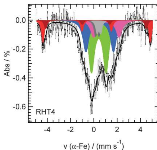
Fig. 7 Deconvoluted Mössbauer spectrum of the sample identified as RHT4 in Fig. 6a and b, i.e. the catalyst initially containing 0.20 wt% Fe of Fig. 6 and which has been submitted to four acid washing steps, each followed by a re-heat-treatment.
