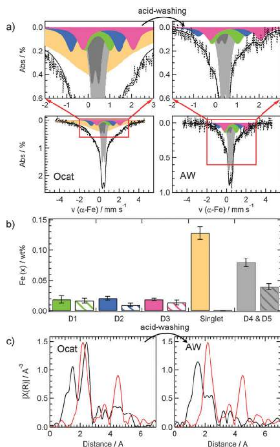
Fig. 5 Effects of acid-washing on the Fe-species in the catalyst containing 0.27 wt% Fe: (A) displays the Mössbauer spectra of the original catalyst (Ocat) and its acid-washed derivative (AW); the full bars in (B) correspond to the iron concentrations of each Fe-species in the Mössbauer spectra of the Ocat, while the patterned bars represent the concentrations in the AW sample; (C) shows the corresponding EXAFS spectra of the original catalyst Ocat and its acid-washed derivative AW. The red lines in both EXAFS spectra are that of an iron foil. The Fe content of the AW catalyst is 0.09 wt%.
