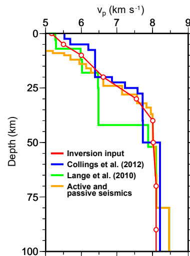
Figure 3. Velocity models used as starting model for the two-dimensional tomographic inversion of v_p (red line and red circles). Because of the large number of stations and events on or near the SFZ, the minimum 1-D velocity model (green line) is dominated by the crustal structure of the Sumatran mainland. This velocity model is not appropriate for the events in the outer forearc, so we constructed a layered 1-D v_p velocity function based on an active source refraction study (Vermeesch et al., 2009). Above 30 km depth, we adopted a one-dimensional, staircase-like velocity–depth function based on an active source refraction study (Vermeesch et al., 2009, orange line); for depths greater than 30 km we adopted the one-dimensional velocity function from a minimum 1-D velocity model (Lange et al., 2010). The blue line shows the minimum 1-D v_p velocity model from Collings et al. (2012) for the region adjacent to the southeast of our study region but covering a similar part of the subduction system.
