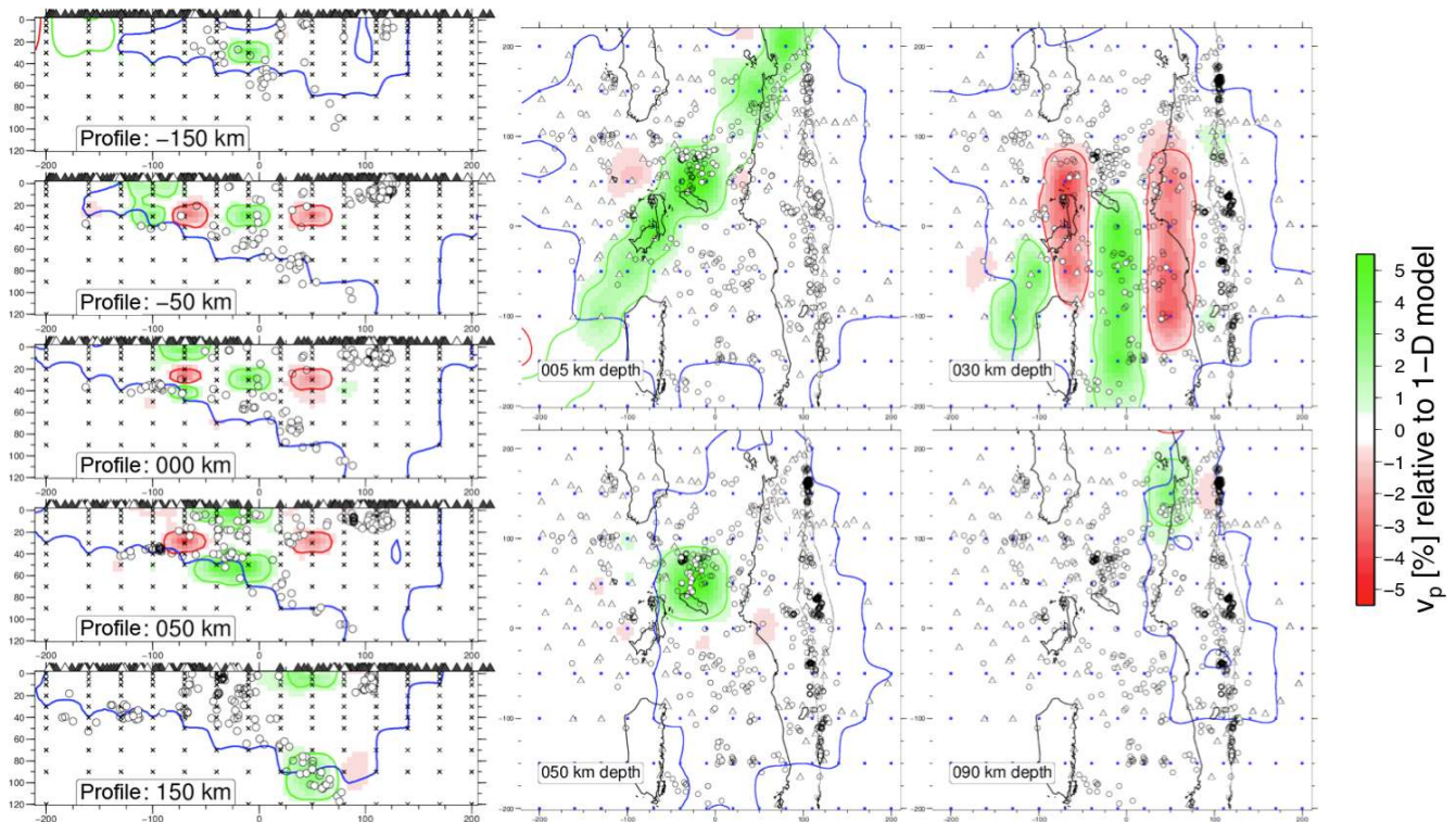
Figure 7. 3-D synthetic models with 5 % velocity v_p perturbation input anomalies and the inversion restoration. The model consists of north–south trending anomalies (map view 30 km depth) and a NE–SW trending low velocity anomaly for both the shallow part of the model in 5 km and for the trace of the subducted IFZ. Red and green lines indicate the 5 % contour lines of the input anomalies. The blue lines encircle regions with good resolution defined by the spread value. Other symbols as in Fig. 5.
