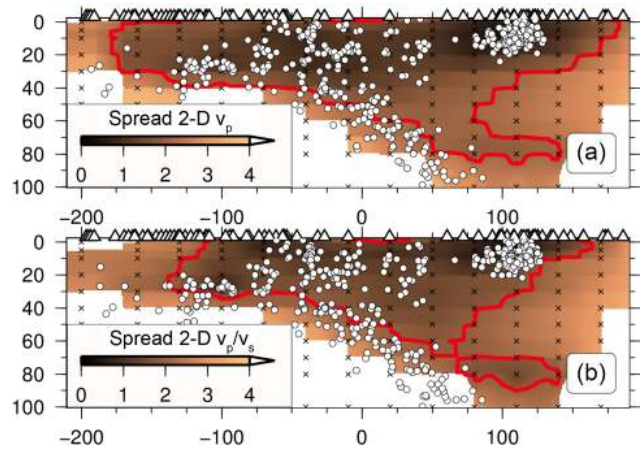
Figure 4. Spread values of 2-D v_p (a) and v_p/v_s (b) inversion. Regions with low spread values and thus good resolution (selection of a cut-off spread value based on analysis of the model resolution matrix and synthetic tests) are encircled with a red line. Cut-off spread values are 2.1 and 1.9 for v_p and v_p/v_s , respectively. Circles indicate hypocenters and grid nodes are shown with crosses. Stations are indicated with triangles.
