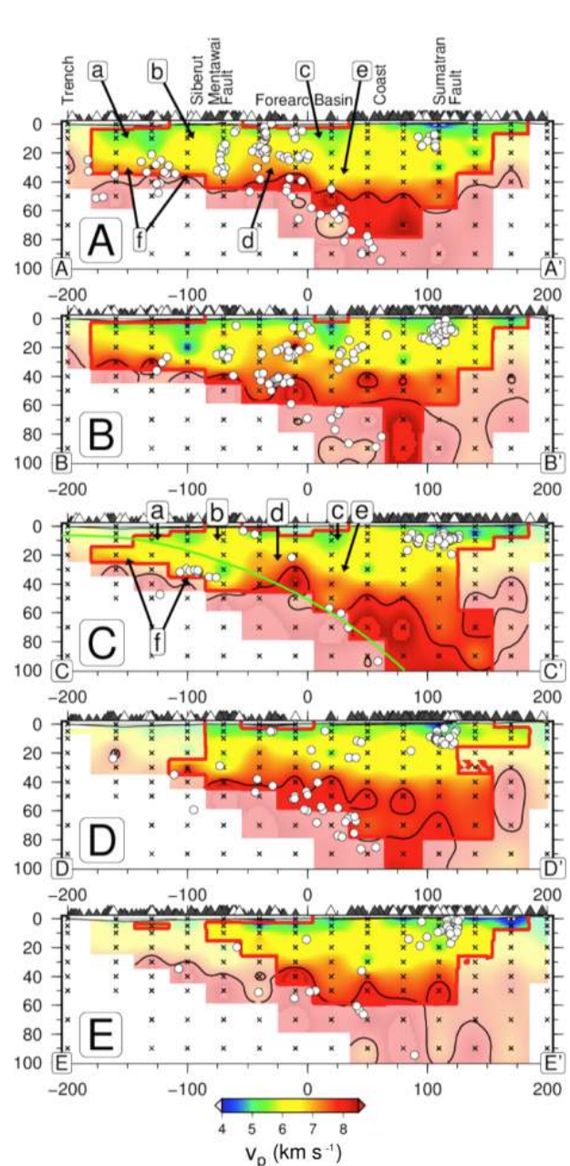
Figure 10. Cross sections along trench-perpendicular trending profiles through the 3-D v_p model. See Fig. 9a for location of cross sections. White circles indicate events within 10 km of the profile and stations closer than 25 km to the profile are shown by white triangles, the remaining ones by black triangles. The 46 OBS stations of the 2-week deployment are shown with smaller triangles. Grid nodes are shown with crosses. Red lines encircle regions of good resolution defined by a cut-off spread value of 1.5. Green line in panel (c) indicates the plate interface as defined by the global SLAB1.0 model (Hayes et al., 2012). The 7.8 \text{km s}^{-1} v_p contour line is indicated by a black line. See text for explanation of characters. Other symbols as in Fig. 6. Note that the geographic labels at the top refer to all profiles, but that only profiles C (Batu Islands) and E (Siberut) actually cross a forearc island.
