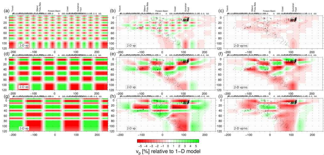
Figure 5. 2-D synthetic checkerboard models with 5 % velocity perturbation input anomalies ( a, d, g ), the inversion restoration for v_p ( b, e, h ) and v_p/v_s ( c, f, i ) models. Crosses represent nodes used in the inversion and the reconstructions are plotted with the resulting hypocenter locations (black points). We calculated different checkerboard inversions using 1 \times 1 and 2 \times 2 (shown in the rows from top to bottom) grid node model perturbations. Noise was added to the synthetic data depending on the quality of the arrivals.
