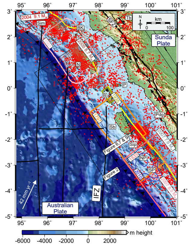
Figure 1. Map showing the tectonic setting of the central Sumatran subduction zone. The locations of earthquakes are indicated by red circles (NEIC catalogue, M \geq 6 , 1 January 1990 until 1 September 2017). The Mentawai Fault (Diament et al., 1992; green line offshore) and the Sumatran Fault (Sieh and Natawidjaja, 2000; black line onshore) are also shown. Bathymetry and topography from the SRTM Plus database (Becker et al., 2009). Oceanic fracture zones from Cande et al. (1989) and Tang et al. (2013). Rupture zones of the great 1797 and 1833 earthquakes are based on uplift of coral microatolls (Natawidjaja et al., 2006). Rupture areas of the 1861, 1935 and 1984 earthquakes are given by Rivera et al. (2002). Slip distribution of the 2004 earthquake from Chlieh et al. (2007). Slip distribution of the 2005 and 2007 earthquakes from Konca et al. (2007, 2008). Convergence between the Australian plate and the forearc sliwer from McNeill and Henstock (2014). Volcanoes (Smithsonian Institute) shown with red triangles. Black boxes indicate locations of Figs. 2, 6, 7 and 9. Abbreviations: Sim: Simeulue; BK: Banyak Islands; Tb: Toba; N: Nias; B: Batu Islands; P: Pulau Pini; Sb: Siberut Island; Sip: Sipora; NP: North Pagai; SP: South Pagai; Pdg: Padang.
