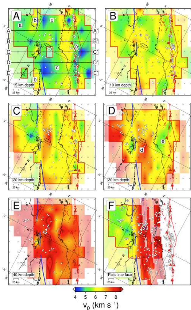
Figure 9. The 3-D v_p model: depth sections (a–e) and curved section along the plate interface as defined by the global SLAB1.0 model (Hayes et al., 2012) (f). Red lines encircle regions of good resolution defined by a cut-off spread value of 1.5. White circles indicate events within 10 km of the section depth, except (f), where all events used for the inversion are shown. Volcanoes (Smithsonian Institute) shown with red triangles. The Mentawai Fault (blue line offshore) and the Sumatran Fault (red line onshore) are also shown. See text for explanation of characters. Other symbols as in Fig. 6.
