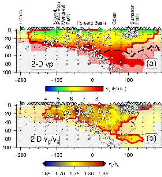
Figure 8. 2-D tomographic velocity models for v_p (a) and v_p/v_s (b) models (profile direction is trench perpendicular). Regions with good resolution are encircled with a red line. Circles indicate hypocenters and grid nodes are shown with crosses. Stations are indicated with triangles. The dashed line in panel (a) indicates the v_p 7.8 \text{ km s}^{-1} contour line and is used as a proxy for the Moho.
