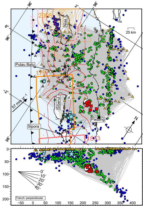
Figure 2. Station and event distribution, and ray coverage of the inversion. Green circles indicate events used in the inversion and corresponding ray paths are indicated by grey lines. Blue circles indicate the complete local catalogue (e.g., with events outside the network, or excluded for other reasons such as large RMS or a small number of picks per event). Yellow triangles (grey triangles for 2-week OBS deployment) indicate stations used in the study. The global Centroid-Moment-Tensor (gCMT) focal mechanism of the 30 September 2009 Padang earthquake and its aftershocks (McCloskey et al., 2010) are indicated in red. The plate coupling from Chlieh et al. (2008) is indicated with red contour lines and labeled with the coupling degree. Light blue squares show the events from the seismic crisis during 2008 occurring in a persistent seismicity cluster SE of Siberut Island (Wiseman et al., 2011), including the M_w 7.2 main shock of 25 February (blue star). Other symbols as in Fig. 1.
