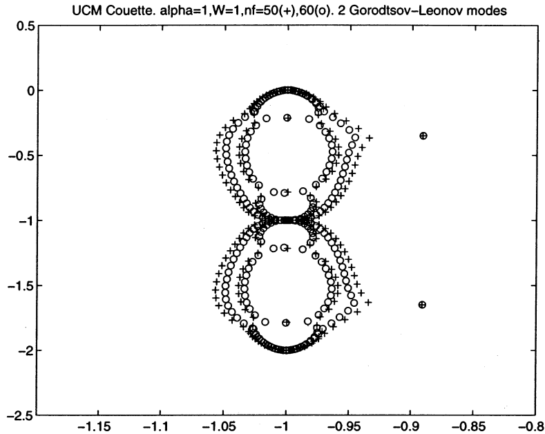
Fig. 2. Eigenspectrum for Couette flow of a UCM fluid using 50 and 60 Chebyshev modes.
