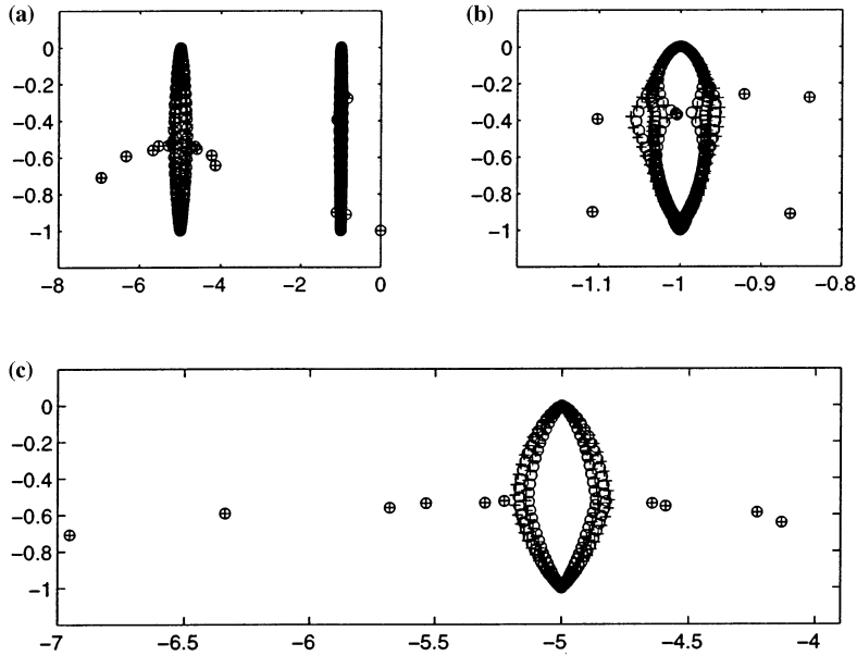
Fig. 6. Spectrum for Poiseuille flow of an Oldroyd-B fluid. (a) shows the entire spectrum; (b) and (c) show the 'UCM' and 'new' parts. The parameters are \alpha = 1 , \beta = 0.2 . Results are shown for 80 (crosses) and 90 (circles) Chebyshev modes.
