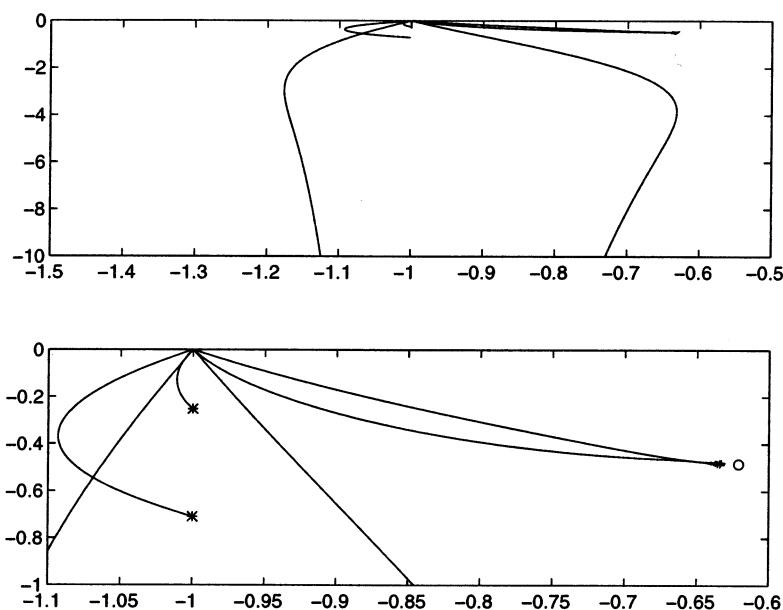
Fig. 7. Motion of the eigenvalues in the \sigma -plane as \alpha varies: Poiseuille flow of a UCM fluid with W = 1 . All eigenvalues coincide at -1 at \alpha = 0 . As \alpha increases, two eigenvalues move to the Gorodtsov-Leonov eigenvalue marked by a circle, two disappear in the continuous spectrum (marked by a star), and two behave like -\alpha - 1/W .
