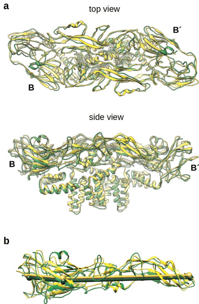
Extended Data Figure 7 | The ectodomain of the ZIKV B-B' dimer is positioned lower in the radius compared to DENV2. a , Top panel shows the top view of the B-B' dimer of ZIKV (green) and DENV2 (yellow), while the bottom panel shows the side view. The position of stem and transmembrane regions in both ZIKV and DENV are similar. b , The ZIKV E ectodomain is positioned at a slightly lower radius than DENV2. Stick connecting similar atoms in ZIKV and DENV is shown to help with the comparison of the positions of the E ectodomains.
