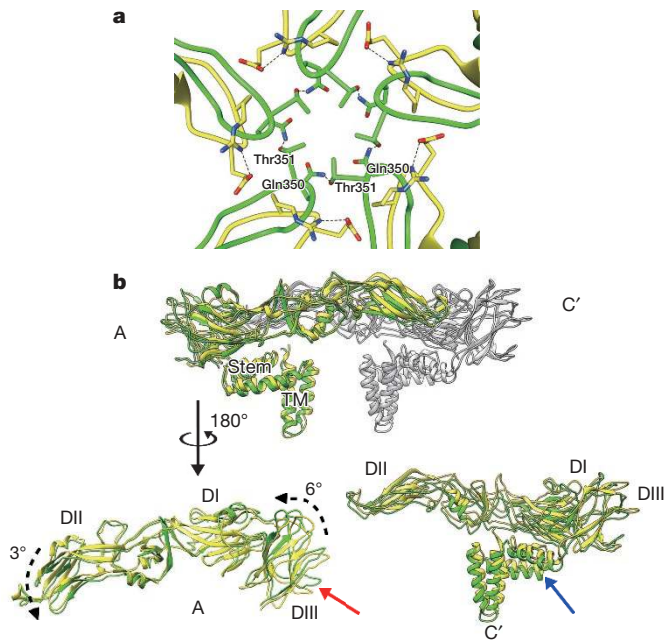
Figure 3 | Possible interactions between the ZIKV DIII CD-loops around the five-fold vertex may cause differences in the position of A–C' dimer compared to DENV2. a , The CD-loops of ZIKV (green) are stretched closer towards the five-fold vertex than those in DENV2 (yellow). In ZIKV, the Gln350 residue may form a hydrogen bond (dashed line) to the Thr351 from the CD-loop of a neighbouring DIII, creating a hydrogen bond network around the five-fold vertex. The DENV2 residues in the CD-loop (yellow), in comparison, do not interact with other neighbouring CD-loops. b , Positional differences of ZIKV A–C' dimer compared to DENV2. Top panel shows the side view. ZIKV and DENV2 molecule A are coloured green and yellow, respectively. Molecule C' of both ZIKV and DENV2 is coloured grey. Bottom left panel shows molecule A rotated by 180° to an axis perpendicular to the viral membrane. The ZIKV CD-loop (red arrow) is lifted upwards probably owing to the five-fold interaction as demonstrated in a ; this molecule rotates slightly. Bottom right panel shows molecule C' in the same orientation as in the top panel. The whole ZIKV E protein (green) molecule C' is positioned at a lower radius than in DENV2 (yellow). The positions of the ZIKV stem (blue arrow) and transmembrane (TM) regions suggest that the membrane is pushed downwards compared to DENV2.
