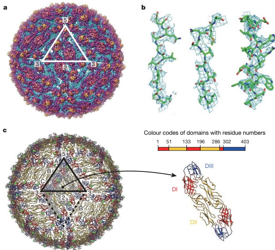
Figure 2 | The 3.7 Å resolution cryoEM structure of ZIKV. a , The ZIKV cryoEM map. The map is coloured radially: 0–219 Å (cyan), 220–240 Å (purple) and >240 Å (gold). b , Zoomed-in view of the density map (cyan mesh) fitted with the E protein structure. c , The E protein arrangement
