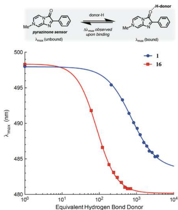
Figure 5. Titration curves from a colorimetric assay that monitors the blue-shift in \lambda_{\text{max}} of the pyrazinone sensor upon complexation with the HB donor analyte ( 1 or 16 ).
