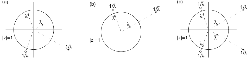
FIG. 7.1. Eigenvalue pairings relative to the unit circle in (a) general bilinear, (b) sesquilinear and (c) real bilinear cases.
