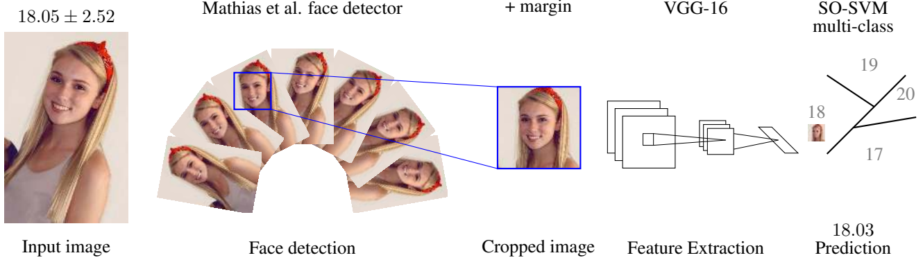
Figure 2. Proposed pipeline for the apparent age estimation.
