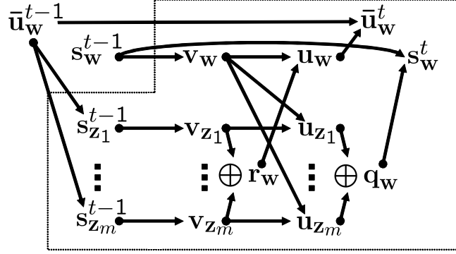
Figure 5: Dependency diagram for memory-efficient dual extragradient. The dotted box represents the computations of an iteration of the algorithm. Only \bar{\mathbf{u}}_w^t and \mathbf{s}_w^t are kept between iterations. Each example is processed one by one and the intermediate results are accumulated as \mathbf{r}_w = \mathbf{r}_w - \mathbf{F}_i \mathbf{v}_{z_i} + \mathbf{f}_i(\mathbf{y}_i) and \mathbf{q}_w = \mathbf{q}_w - \mathbf{F}_i \mathbf{u}_{z_i} + \mathbf{f}_i(\mathbf{y}_i) . Details shown in Fig. 6, except that intermediate variables \mathbf{u}_w and \mathbf{q}_w are only used here for pictorial clarity.
