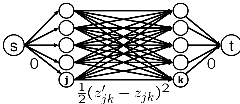
Figure 3: Euclidean projection onto the matching polytope using min-cost quadratic flow. Source s is connected to all the “source” nodes and target t connected to all the “target” nodes, using edges of capacity 1 and cost 0. The original edges jk have a quadratic cost \frac{1}{2}(z'_{jk} - z_{jk})^2 and capacity 1.
