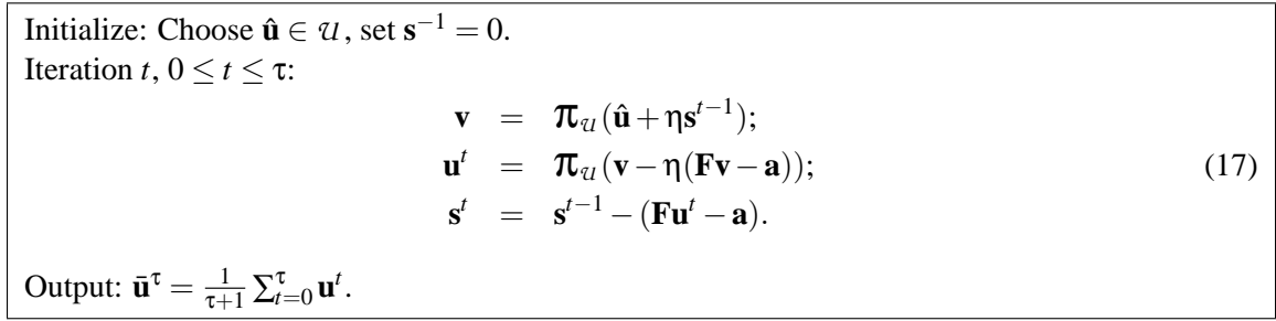
Figure 2: Euclidean dual extragradient.
