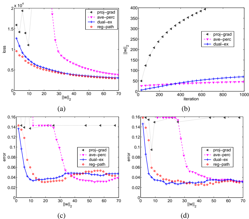
Figure 7: Object segmentation results: (a) Training hinge loss for the regularization path (reg-path), the averaged projected gradient (proj-grad), the averaged perceptron (ave-perc) and unregularized dual extragradient (dual-ex) vs. the norm of the parameters. (b) Norm of the parameters vs. iteration number for the three algorithms. (c) Validation error vs. the norm of the parameters. (d) Test error vs. the norm of the parameters.
