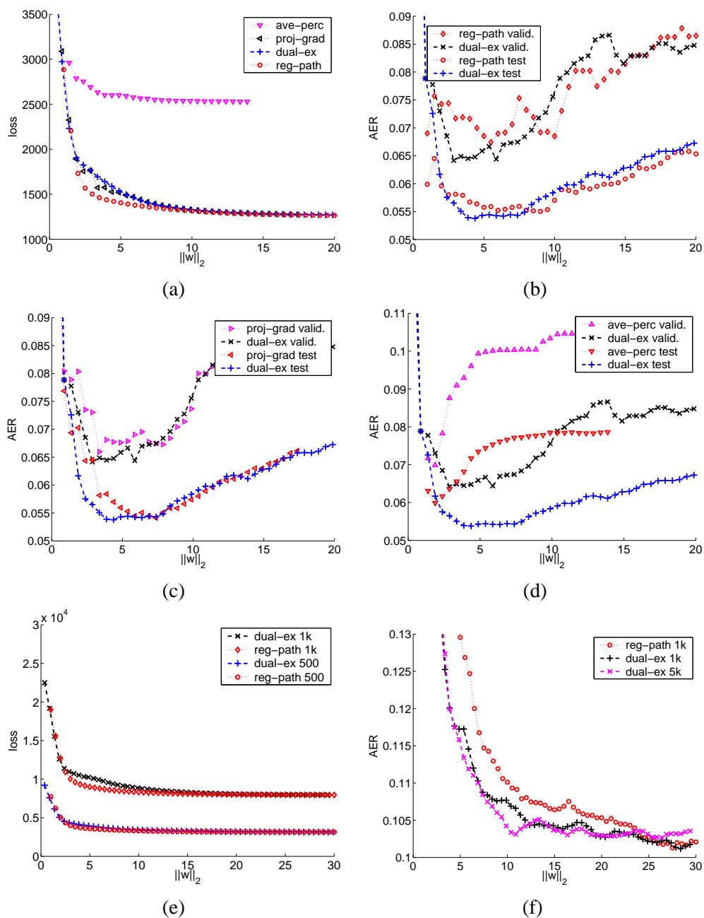
Figure 8: Word alignment results: (a) Training hinge loss for the three different algorithms and the regularization path on the Gold dataset. (b) AER for the unregularized dual extragradient (dual-ex) and the regularization path (reg-path) on the 347 Gold sentences (test) and the validation set (valid) when trained on the 100 Gold sentences; (c) Same setting as in (b), comparing dual-ex with the averaged projected-gradient (proj-grad); (d) Same setting as in (b), comparing proj-grad with the averaged perceptron (ave-perc); (e) Training hinge loss for dual-ex and reg-path on 500 and 1000 GIZA++ labeled sentences. (f) AER for dual-ex and reg-path tested on the Gold test set and trained on 1000 and 5000 GIZA++ sentences. The graph for 500 sentences is omitted for clarity.
