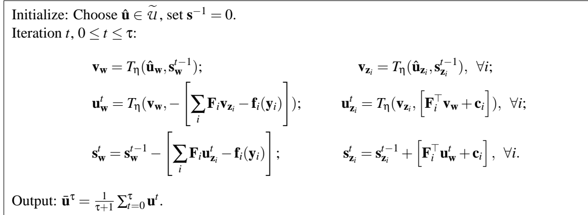
Figure 4: Non-Euclidean dual extragradient.
